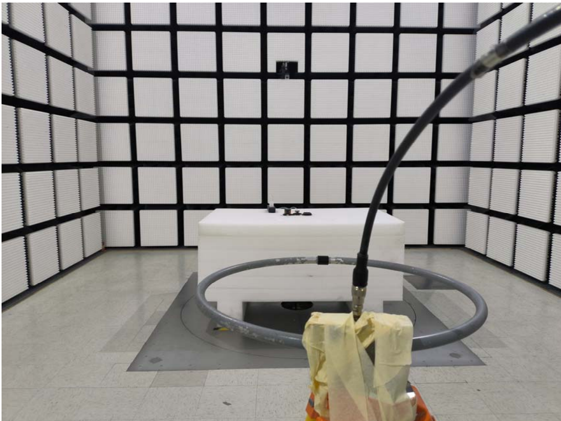
Radiated Emission Below 1GHz Ground-parallel View-M2
