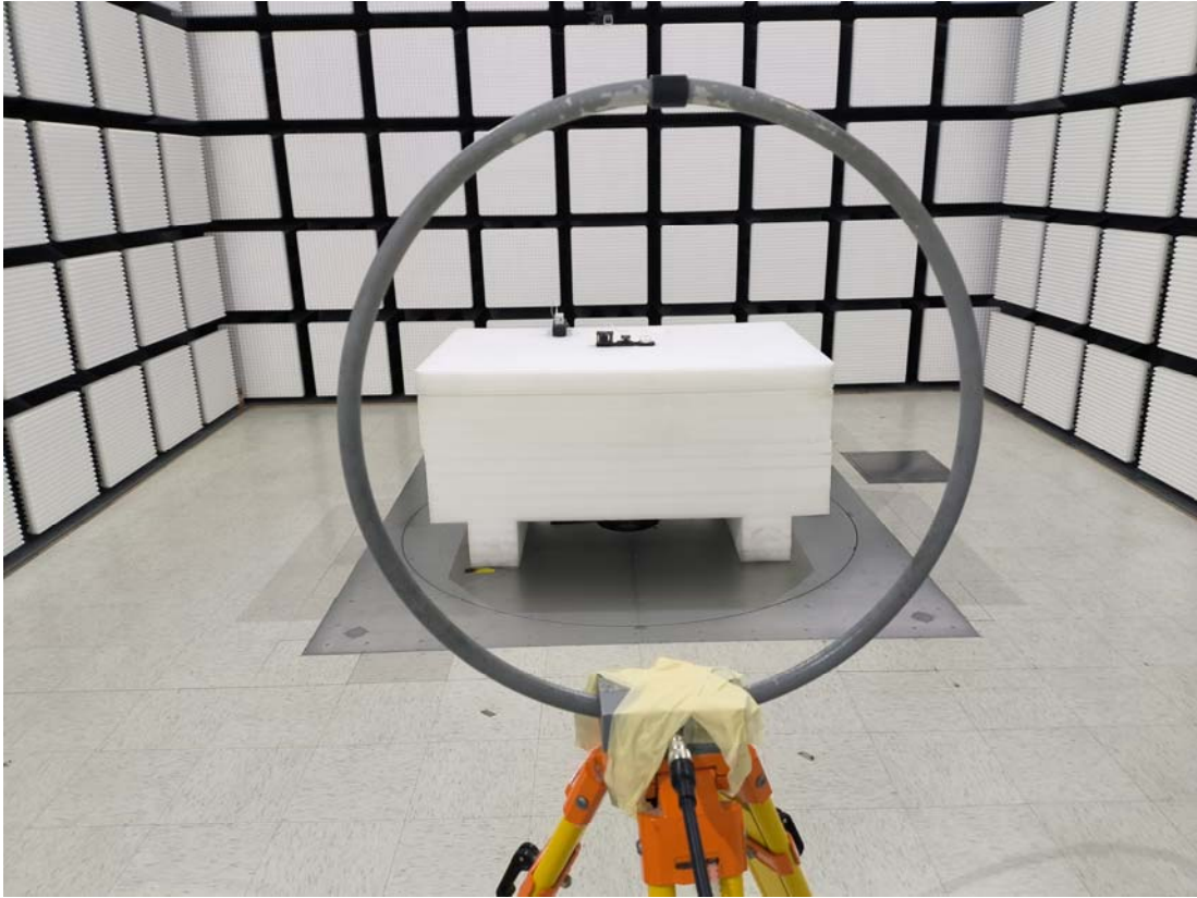
Radiated Emission Below1GHz Parallel View-M1
