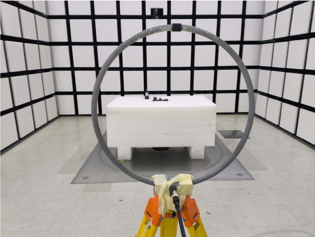
Radiated Emission Below1GHz Parallel View-M2
