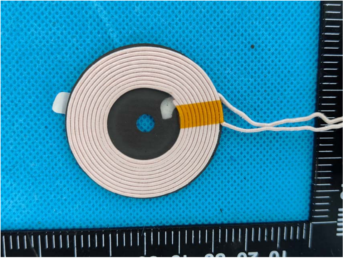
Coil2 15W
