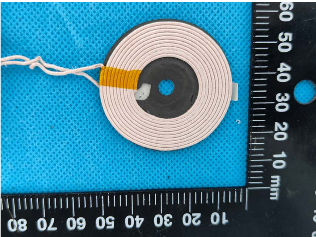
Coil2 15W
