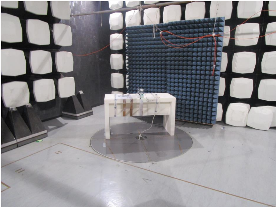
Photograph 3: EUT Test Setup for Electric Field Strength strength under 1GHz
