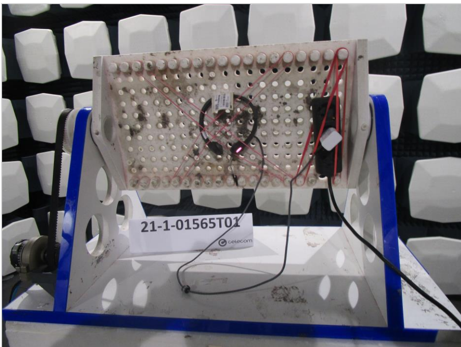
Photograph 3: EUT Test Setup for Electric Field Strength strength above 1GHz strength
