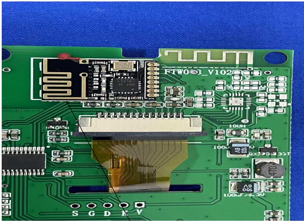
PCB ANTENNA
