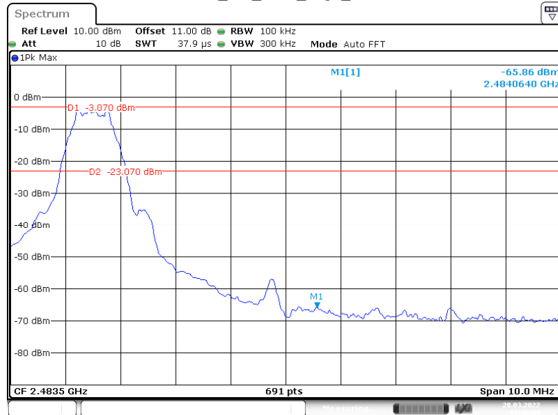
BLE_1M_Ant1_High_2480
