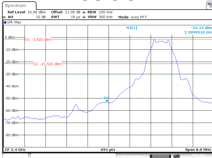
BLE_1M_Ant1_Low_2402
