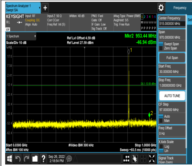
Band26-1.4MHz-16QAM-26697-1RB#0-Range1:30~1000MHz
