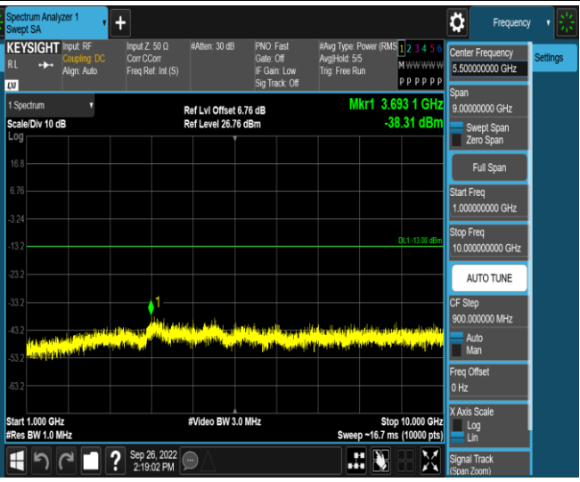
Band26-1.4MHz-16QAM-26697-1RB#0-Range2:1000~10000MHz
