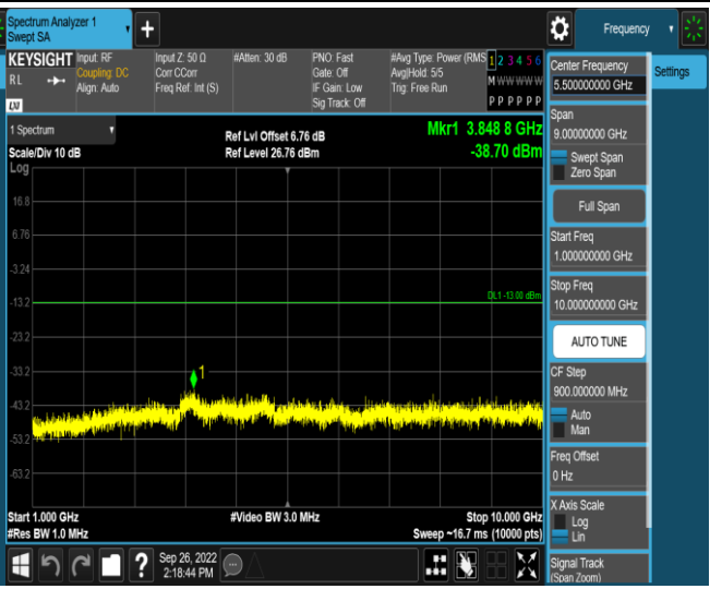
Band26-1.4MHz-QPSK-26740-1RB#0-Range2:1000~10000MHz
