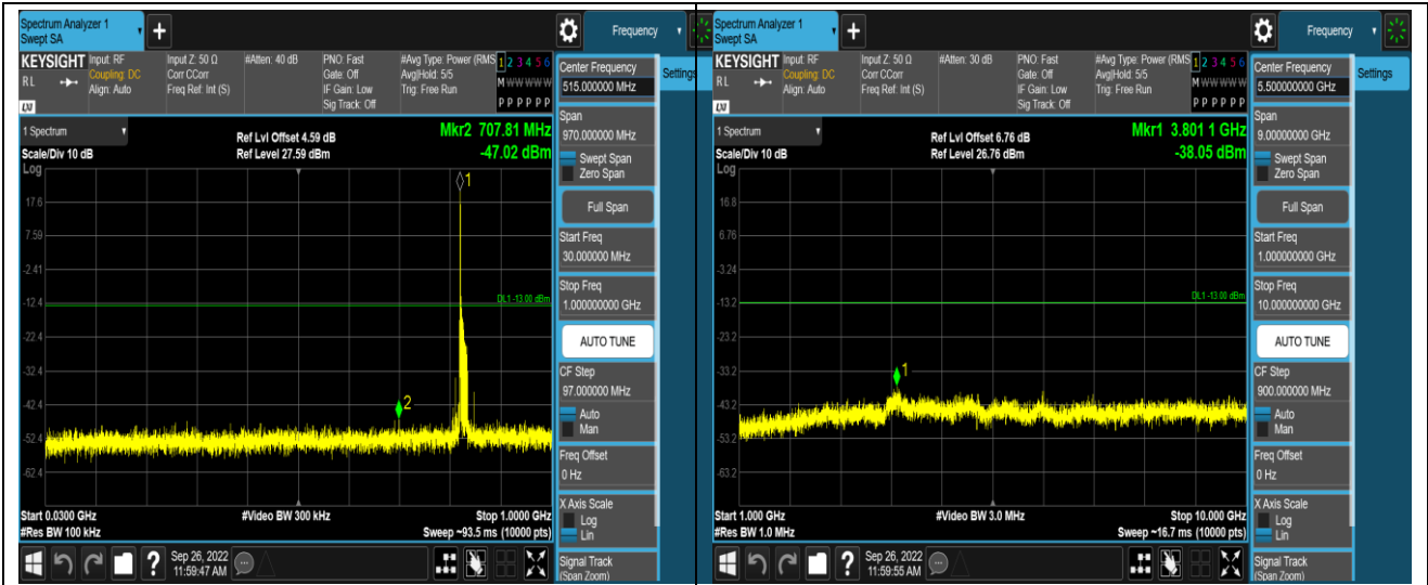
Band26-15MHz-QPSK-26915-1RB#0-Range1:30~1000MHz
