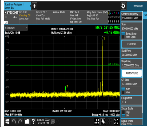
Band26-1.4MHz-16QAM-27033-1RB#0-Range1:30 ~1000MHz
