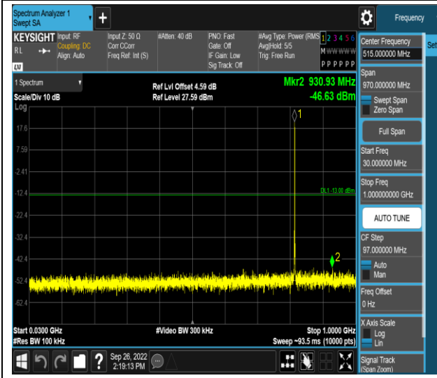
Band26-1.4MHz-QPSK-26740-1RB#0-Range1:30~1000MHz
