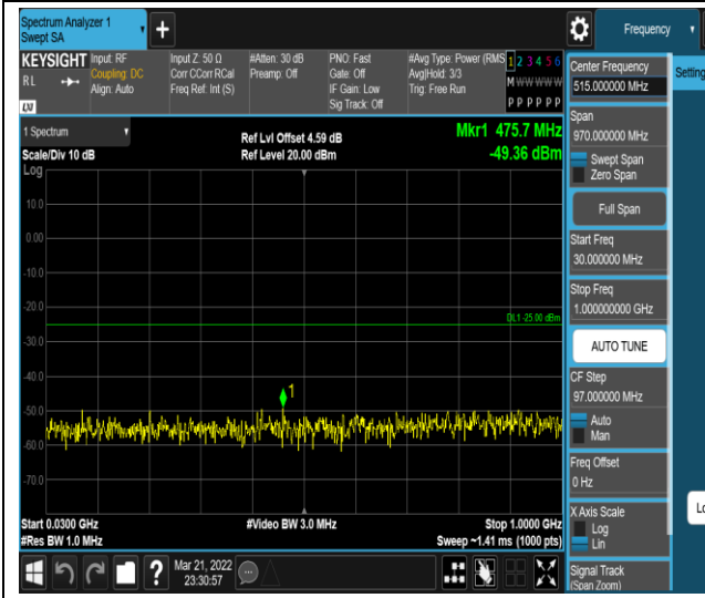
Band38-20MHz-QPSK-37850-1RB#0-Range1:30~1000MHz
