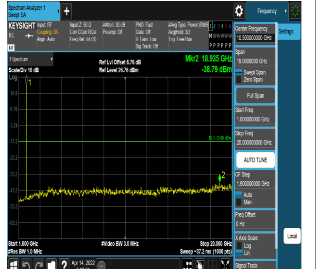
Band66-1.4MHz-16QAM-132322-1RB#0-Range2:100 0~20000MHz
