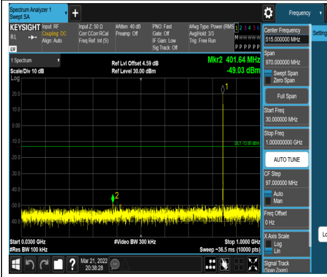
Band5-1.4MHz-QPSK-20643-1RB#0-Range1:30~1000MHz
