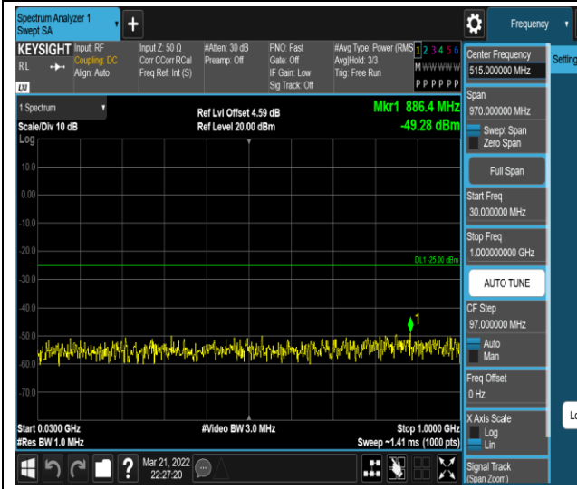
Band7-20MHz-16QAM-21100-1RB#0-Range1:30~1000MHz
