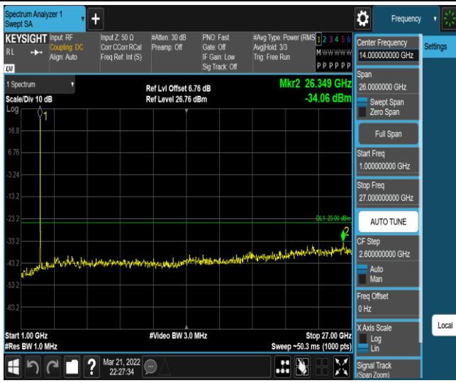
Band7-20MHz-16QAM-21100-1RB#0-Range2:1000~27000MHz
