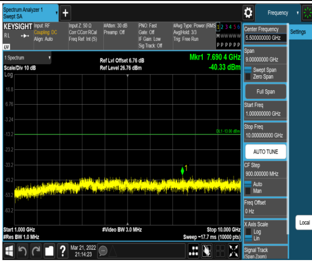
Band5-10MHz-QPSK-20525-1RB#0-Range2:1000~10000MHz
