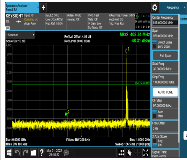
Band5-10MHz-QPSK-20525-1RB#0-Range1:30~1000MHz
