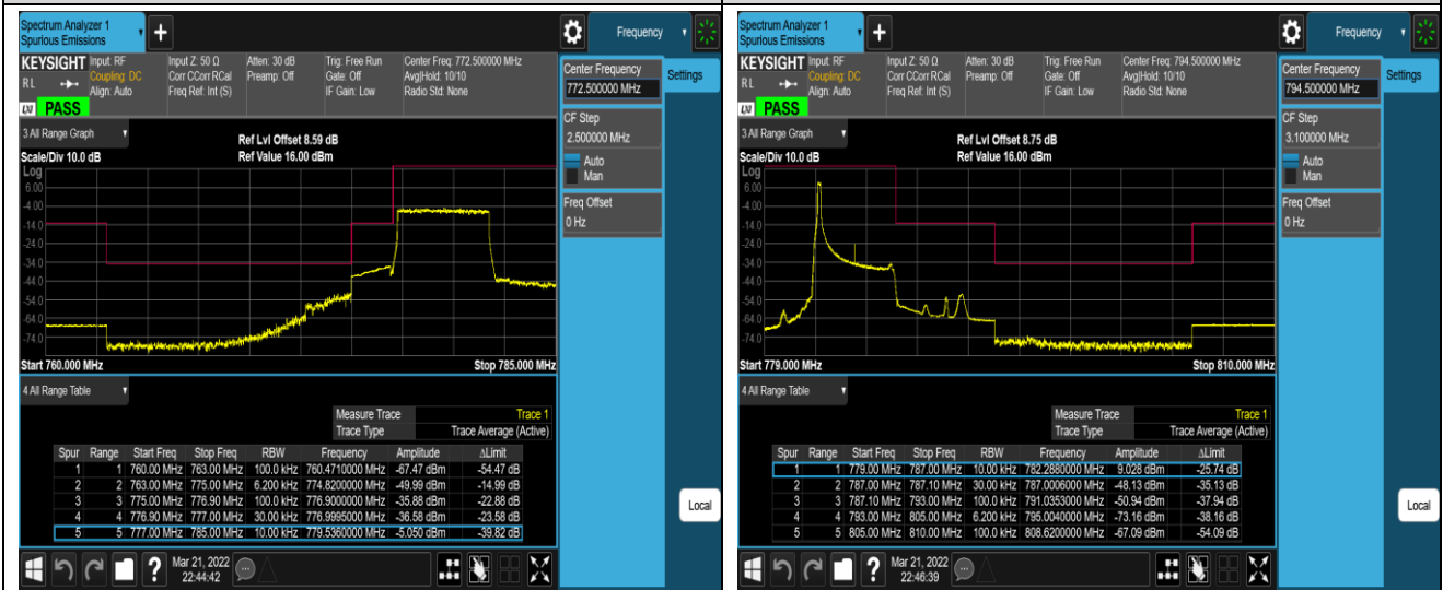
Band13-5MHz-QPSK-23255-1RB#24
