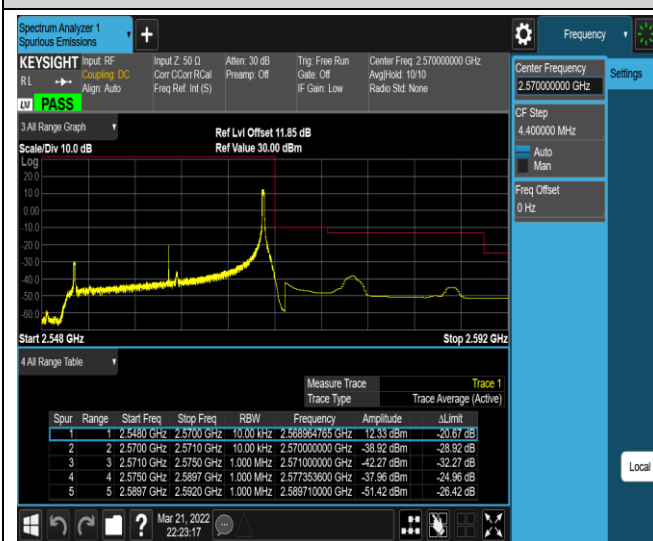
Band7-20MHz-16QAM-2085-1RB#0
