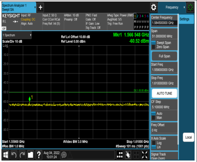
Band13-10MHz-16QAM-23230-1RB#0-Range3:1559 ~1610MHz
