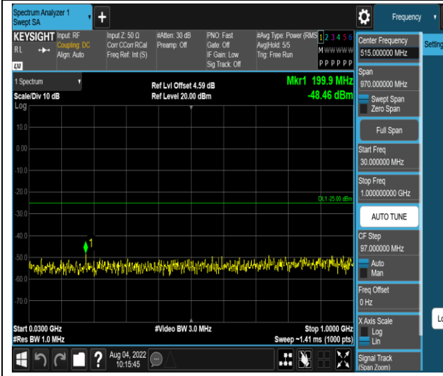
Band41-5MHz-QPSK-41215-1RB#0-Range1:30~1000MHz
