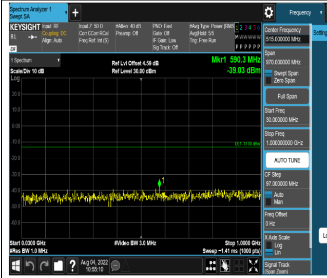
Band66-1.4MHz-QPSK-131979-1RB#0-Range1:30~1000MHz
