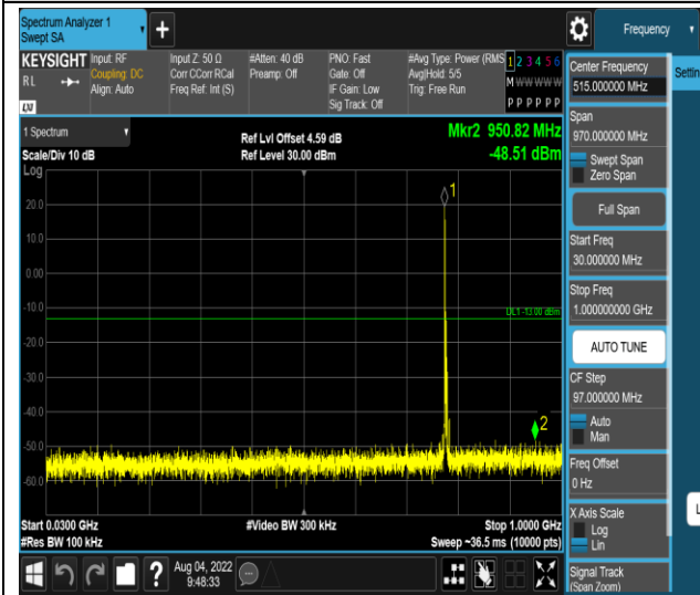
Band13-5MHz-16QAM-23230-1RB#0-Range1:30~1000MHz
