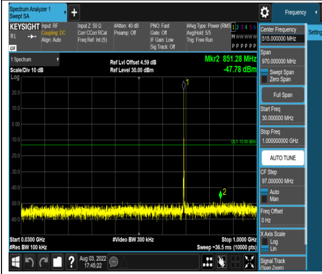
Band12-1.4MHz-16QAM-23017-1RB#0-Range1:30~1000MHz
