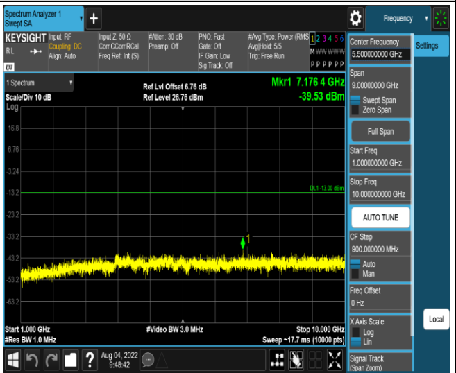
Band13-5MHz-16QAM-23230-1RB#0-Range2:1000~10000MHz
