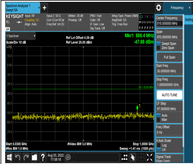
Band7-5MHz-16QAM-21425-1RB#0-Range1:30~1000MHz
