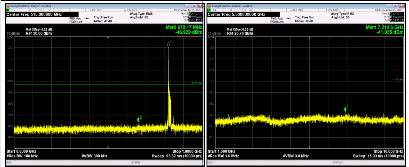
Band26-15MHz-QPSK-26865-1RB#0-Range1:30~1000MHz
