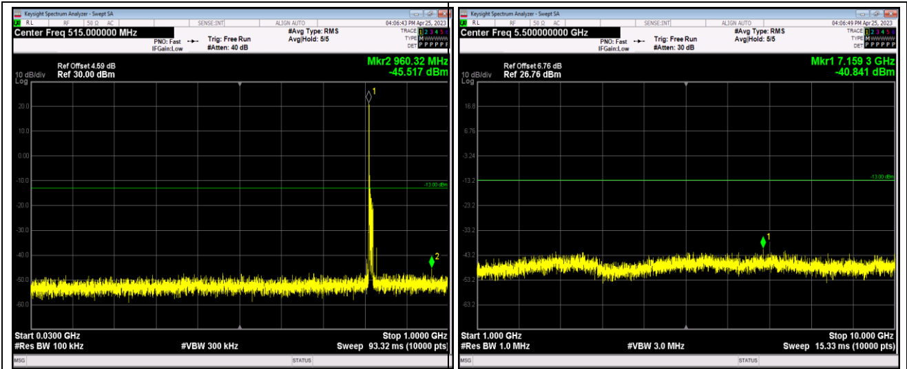
Band26-10MHz-16QAM-26740-1RB#0-Range1:30~1000MHz
