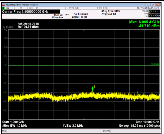
Band17-5MHz-QPSK-23790-1RB#0-Range2:1000~10000MHz
