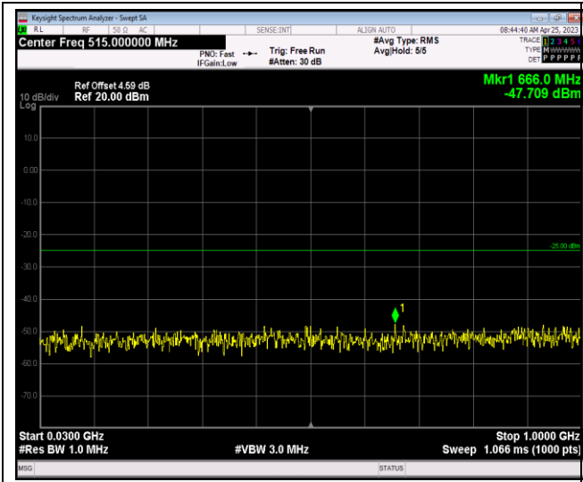
Band7-20MHz-16QAM-21350-1RB#0-Range1:30~1000MHz
