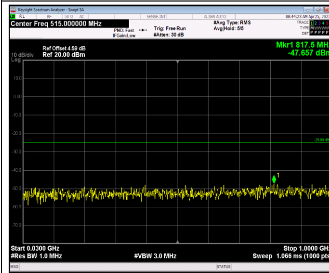
Band7-20MHz-QPSK-21100-1RB#0-Range1:30~1000MHz
