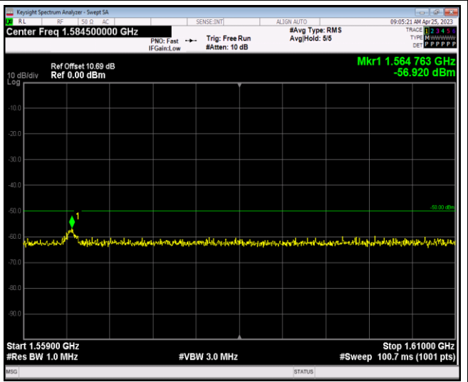
Band13-5MHz-16QAM-23255-1RB#0-Range3:1559~ 1610MHz
