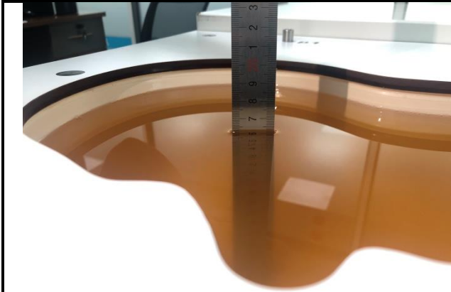
Fig. 9.3 Photo of Liquid Height for Head SAR (600MHz~6000MHz)(depth>15cm)
