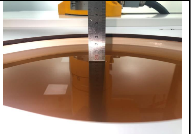
Fig. 9.4 Photo of Liquid Height for Body SAR (600MHz~6000MHz) (depth>15cm)
