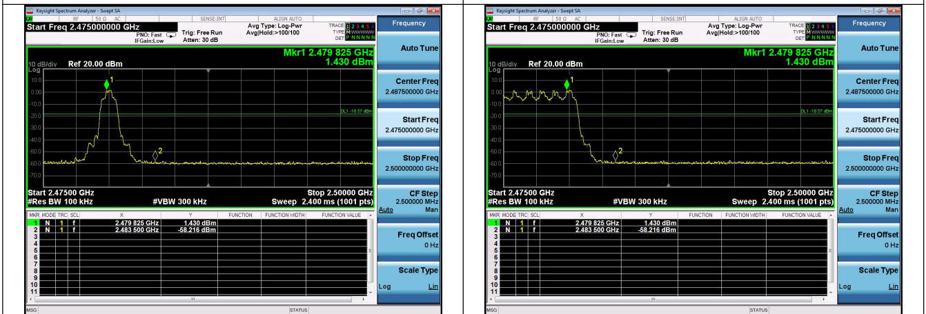
\pi/4 DQPSK No-Hopping Band edge-Right side
