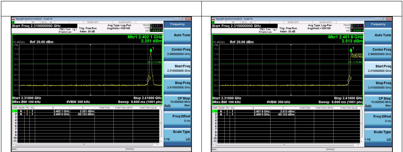
\pi/4 DQPSK No-Hopping Band edge-Left side
