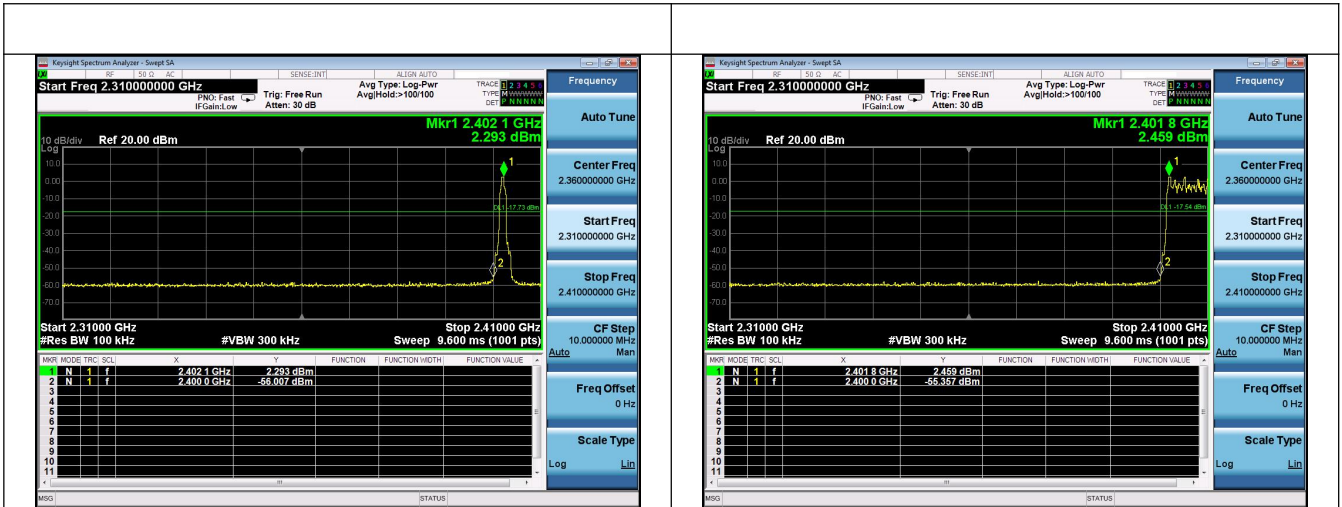
8DPSK No-Hopping Band edge-Left side
