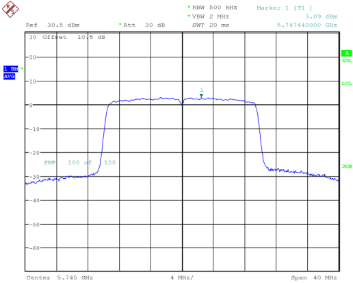
802.11ax20_5745MHz_RU_Full_Chain 0
