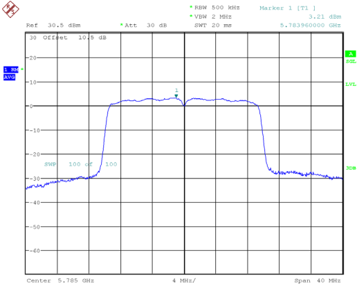
802.11ax20_5785MHz_RU_Full_Chain 0
