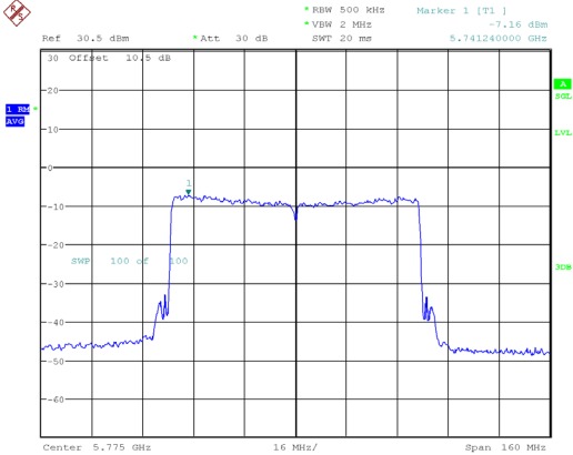
802.11ax80_5775MHz_RU_Full_Chain 1
