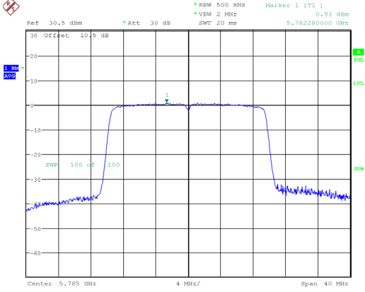
802.11ax20_5785MHz_RU_Full_Chain 1
