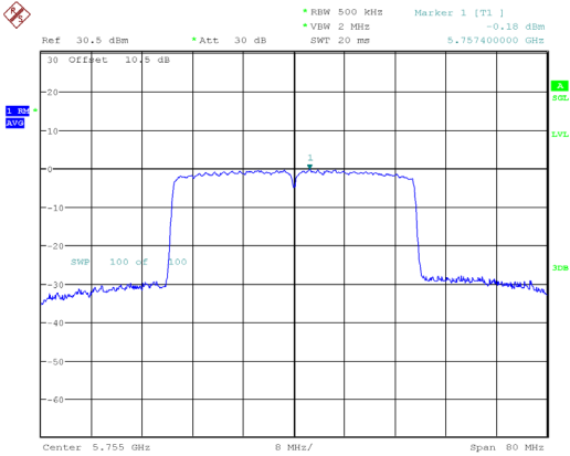
802.11ax40_5755MHz_RU_Full_Chain 0
