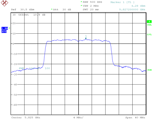
802.11ax20_5825MHz_RU_Full_Chain 1
