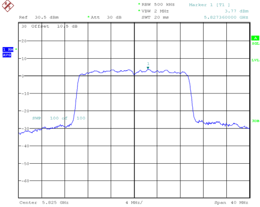
802.11ax20_5825MHz_RU_Full_Chain 0
