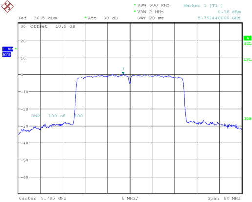
802.11ax40_5795MHz_RU_Full_Chain 0
