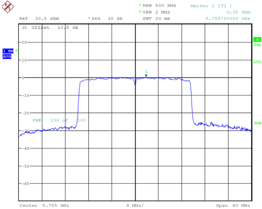
802.11ax40_5755MHz_RU_Full_Chain 1
