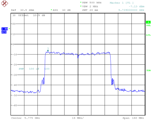
802.11ax80_5775MHz_RU_Full_Chain 0
