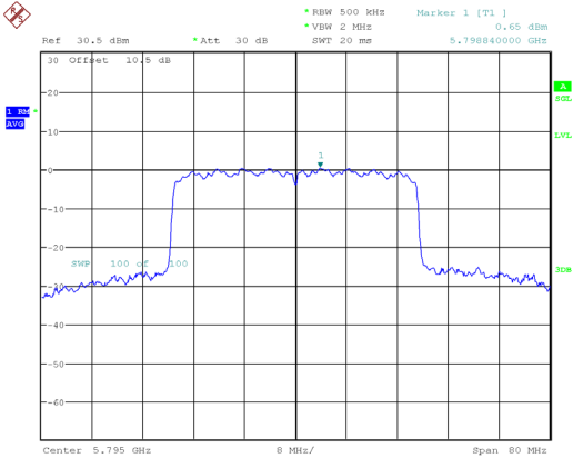
802.11ax40_5795MHz_RU_Full_Chain 1
