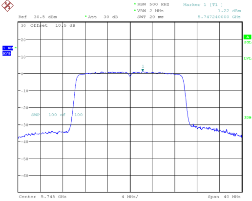
802.11ax20_5745MHz_RU_Full_Chain 1
