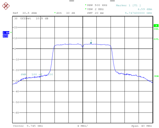
802.11a_5745MHz_Chain 1
