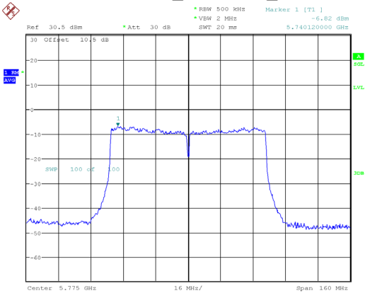
802.11ac80_5775MHz_Chain 1
