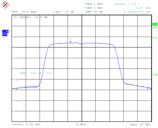
802.11ax20_5320MHz_RU_Full_Chain 1
