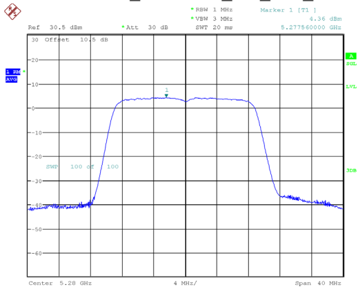
802.11ax20_5280MHz_RU_Full_Chain 0
