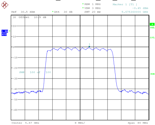
802.11ax40_5670MHz_RU_Full_Chain 0
