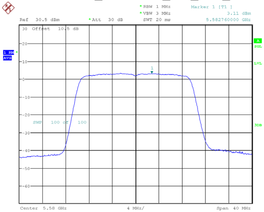
802.11ax20_5580MHz_RU_Full_Chain 1
