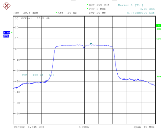
802.11a_5745MHz_Chain 0
