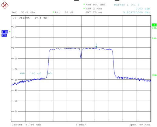
802.11ac40_5795MHz_Chain 0
