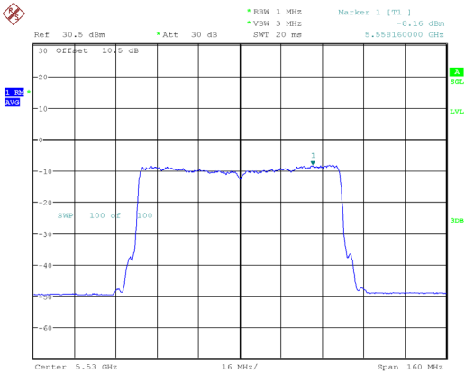
802.11ax80_5530MHz_RU_Full_Chain 1
