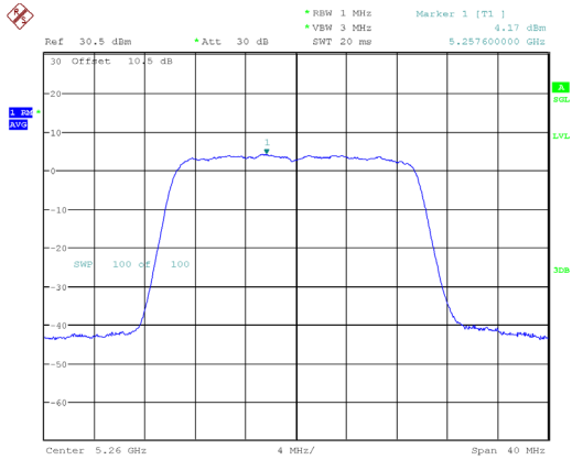
802.11ax20_5260MHz_RU_Full_Chain 1
