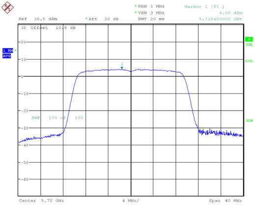
802.11ax20_5720MHz_RU_Full_Chain 0
