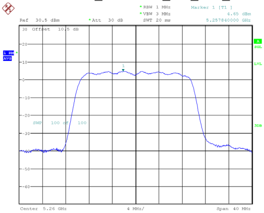
802.11ax20_5260MHz_RU_Full_Chain 0
