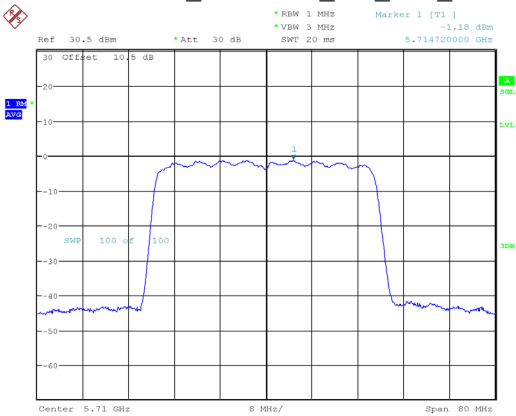
802.11ax40_5710MHz_RU_Full_Chain 0
