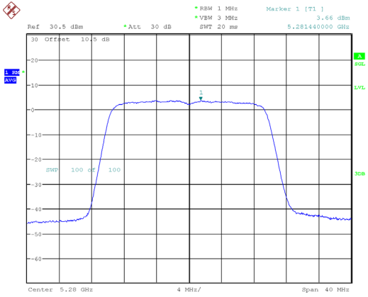
802.11ax20_5280MHz_RU_Full_Chain 1
