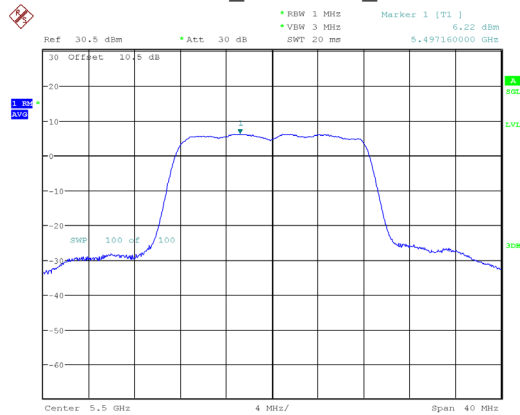
802.11a_5500MHz_Chain 0
