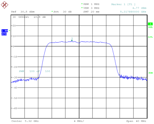
802.11ax20_5320MHz_RU_Full_Chain 0
