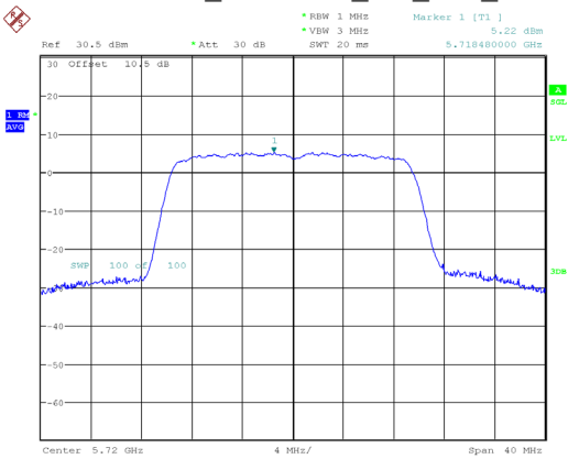
802.11ax20_5720MHz_RU_Full_Chain 1
