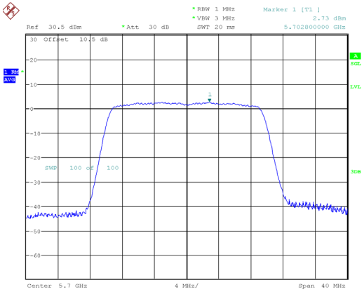
802.11ax20_5700MHz_RU_Full_Chain 0
