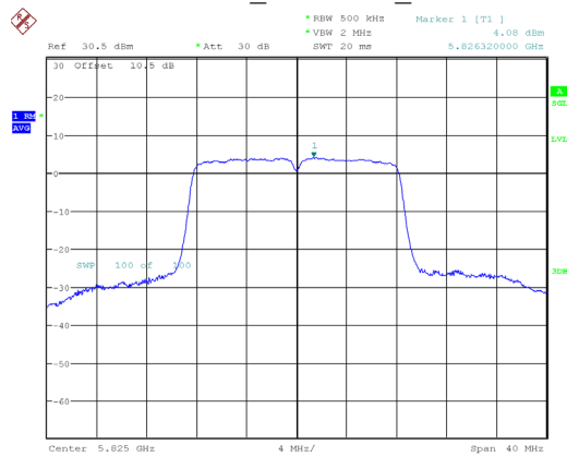
802.11a_5825MHz_Chain 0
