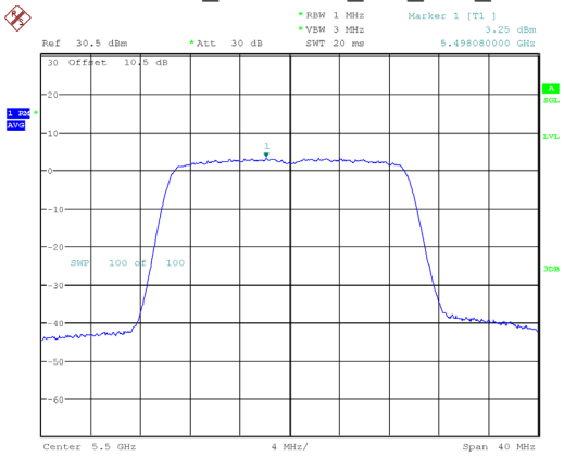
802.11ax20_5500MHz_RU_Full_Chain 0
