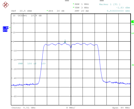
802.11ac40_5510MHz_Chain 0
