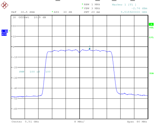
802.11ax40_5510MHz_RU_Full_Chain 0
