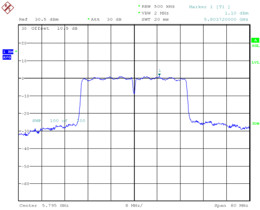
802.11ac40_5795MHz_Chain 1
