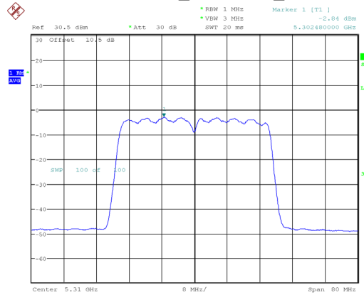
802.11ac40_5310MHz_Chain 1
