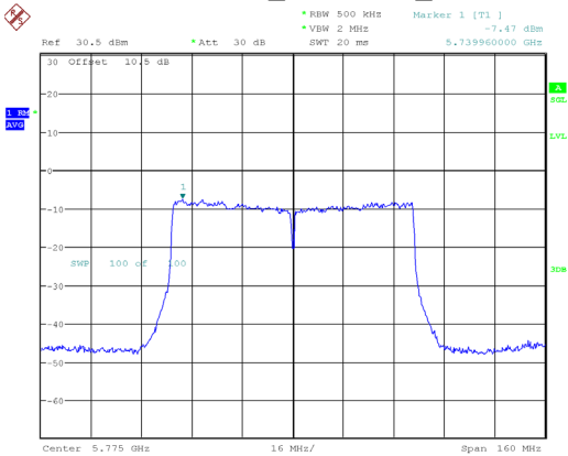
802.11ac80_5775MHz_Chain 0
