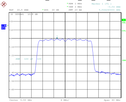
802.11ax40_5550MHz_RU_Full_Chain 0
