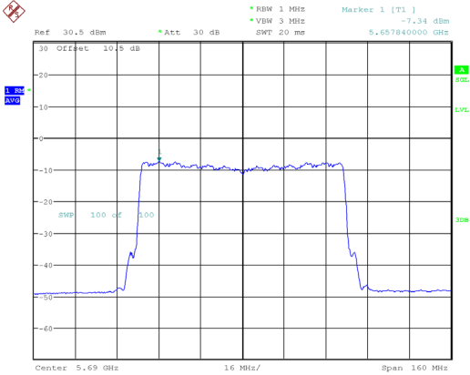
802.11ax80_5690MHz_RU_Full_Chain 1
