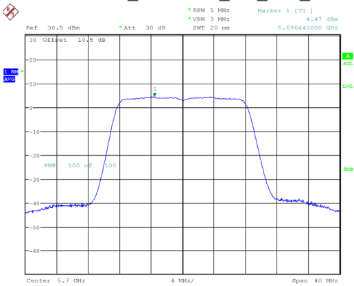
802.11ax20_5700MHz_RU_Full_Chain 1
