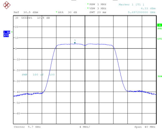
802.11a_5700MHz_Chain 0
