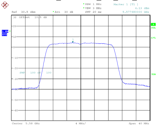
802.11ax20_5580MHz_RU_Full_Chain 0
