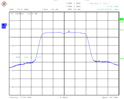
802.11a_5580MHz_Chain 1
