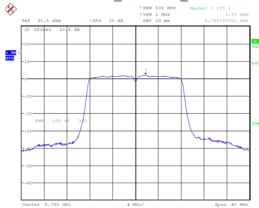
802.11a_5785MHz_Chain 1
