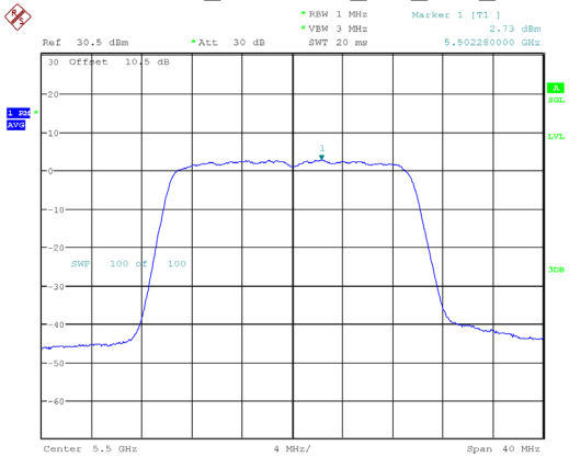
802.11ax20_5500MHz_RU_Full_Chain 1
