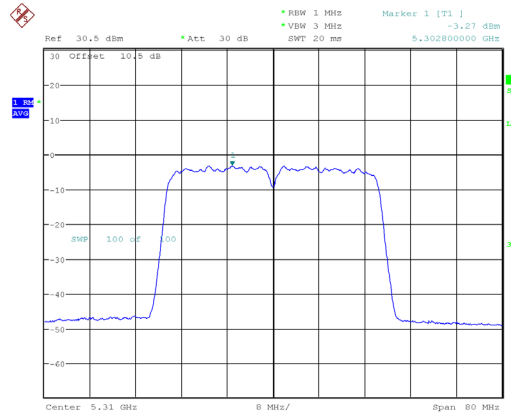
802.11ac40_5310MHz_Chain 0
