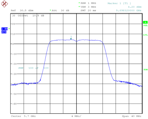
802.11a_5700MHz_Chain 1
