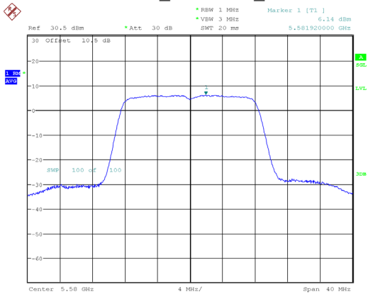
802.11a_5580MHz_Chain 0
