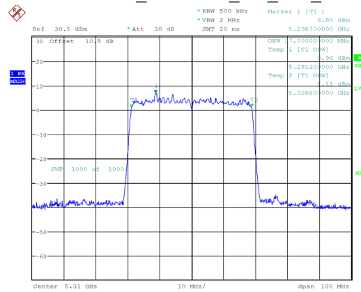
802.11ax40_5310MHz_RU_Full_Chain 0
