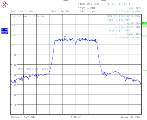
802.11a_5700MHz_Chain 1
