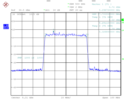
802.11ax40_5310MHz_RU_Full_Chain 1
