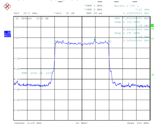
802.11ax80_5290MHz_RU_Full_Chain 1
