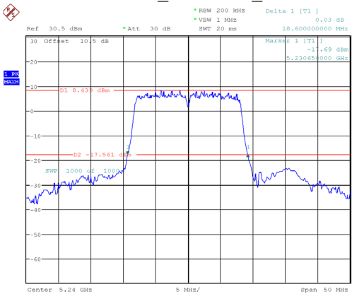
802.11a_5240MHz_Chain 0
