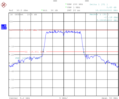
802.11a_5200MHz_Chain 1
