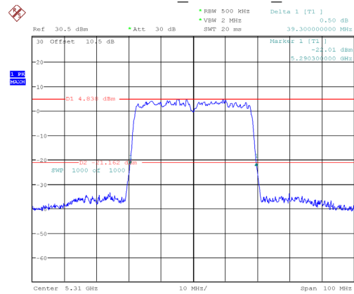
802.11ac40_5310MHz_Chain 0
