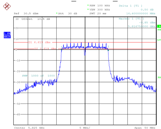
802.11a_5825MHz_Chain 1
