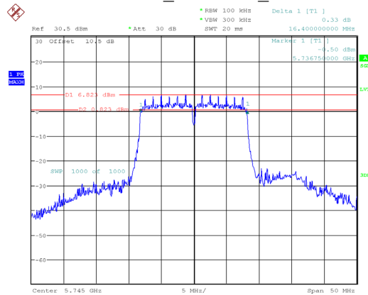
802.11a_5745MHz_Chain 1
