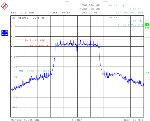
802.11a_5785MHz_Chain 1
