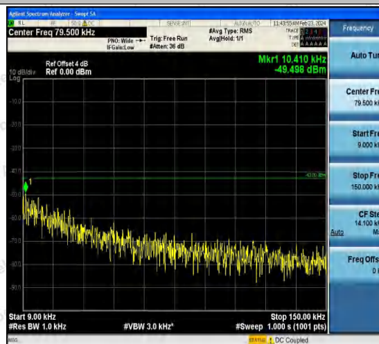
Band2-9538-5-0.009~0.15MHz-PASS
