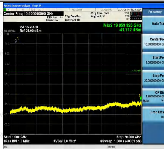
Band2-9400-5-1000~20000MHz-PASS
