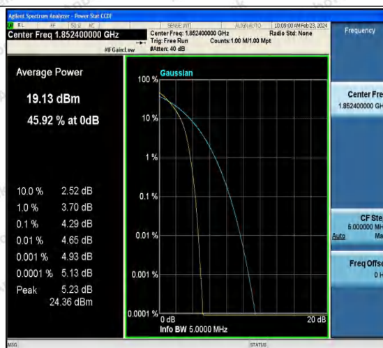
Band2-9262-1-PASS
