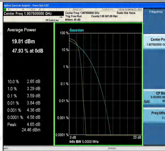
Band2-9538-2-PASS
