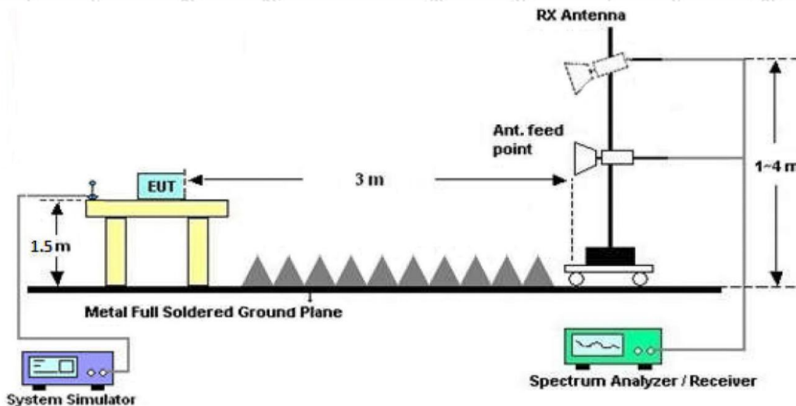
Figure 3. Above 1 GHz
