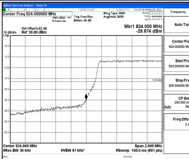
Band5-1.4MHz-16QAM-20643-6RB#0
