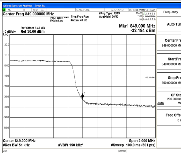
Band5-5MHz-QPSK-20425-25RB#0
