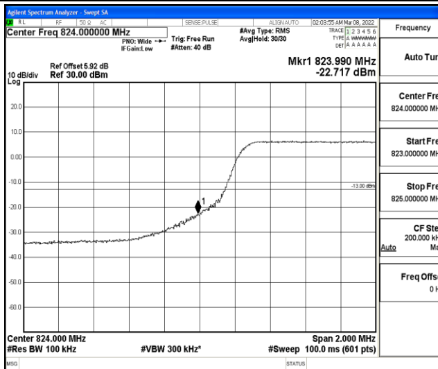
Band5-5MHz-QPSK-20625-25RB#0
