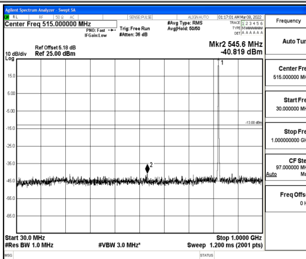
Band5-1.4MHz-QPSK-20407-1RB#0-Range4:1000~10000MHz
