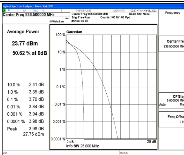
Band5-10MHz-QPSK-20525-50RB#0
