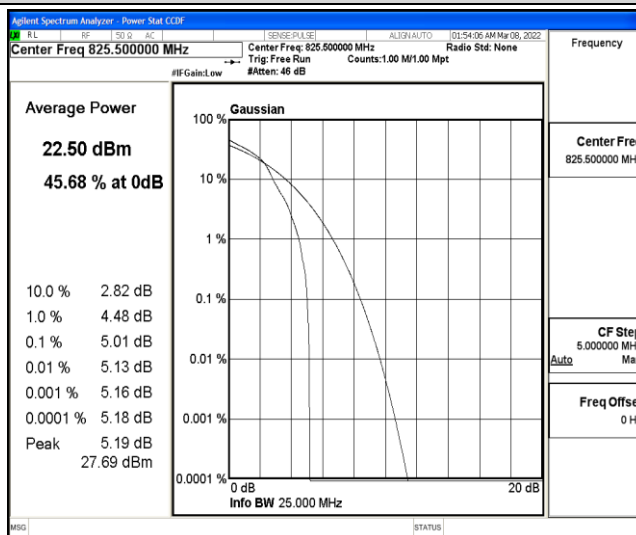
Band5-3MHz-16QAM-20415-15RB#0
