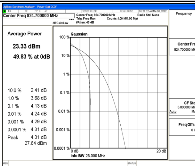
Band5-1.4MHz-QPSK-20407-6RB#0
