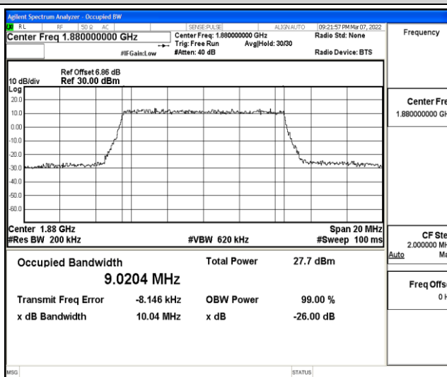
Band2-10MHz-16QAM-19150-50RB#0
