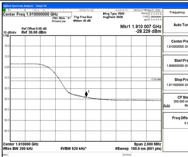
Band2-10MHz-16QAM-18650-50RB#0
