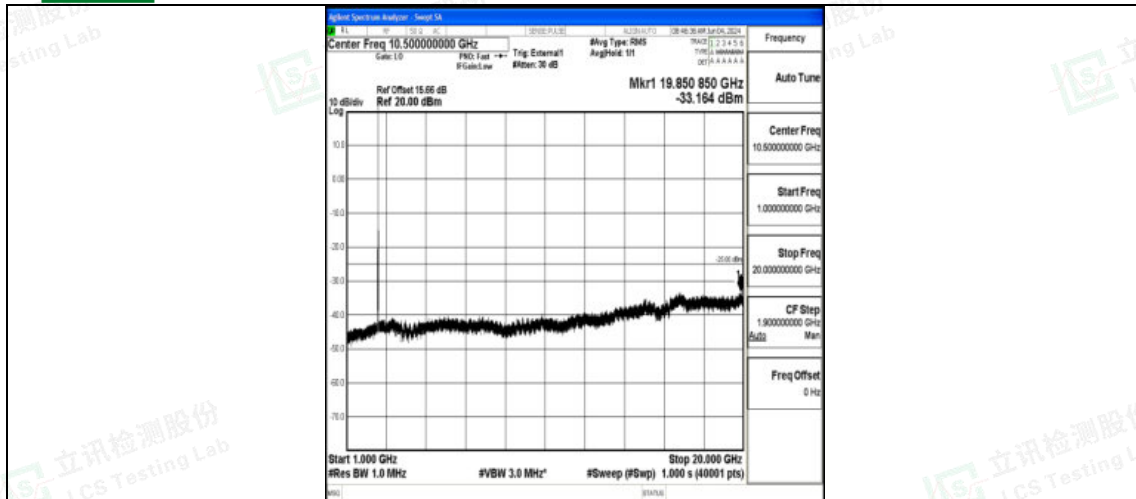
Band41_15MHz_16QAM_39725_1RB#0_1000~20000_1000~20000
