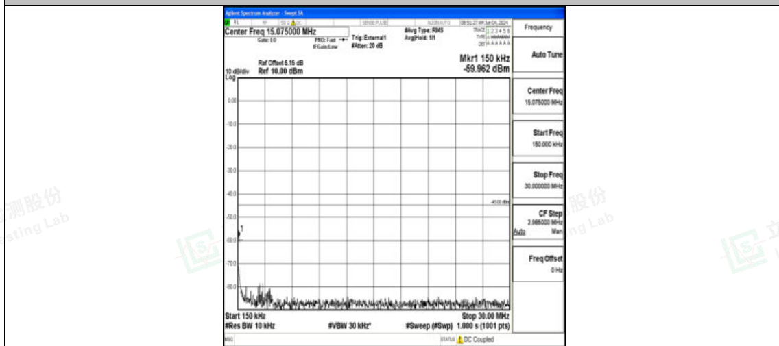
Band41_15MHz_QPSK_41515_1RB#0_0.15~30_0.15~30
