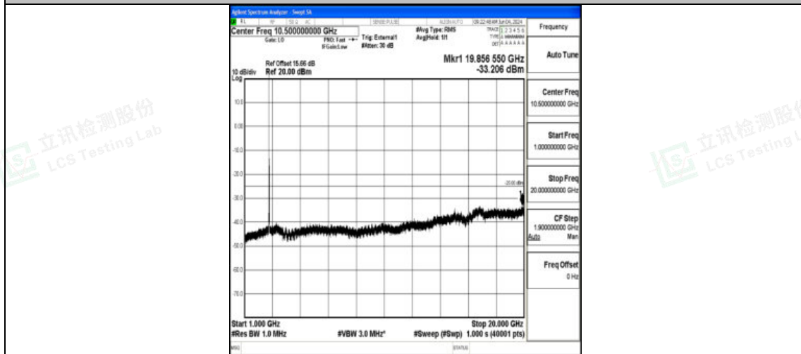
Band41_20MHz_16QAM_41490_1RB#0_1000~20000_1000~20000
