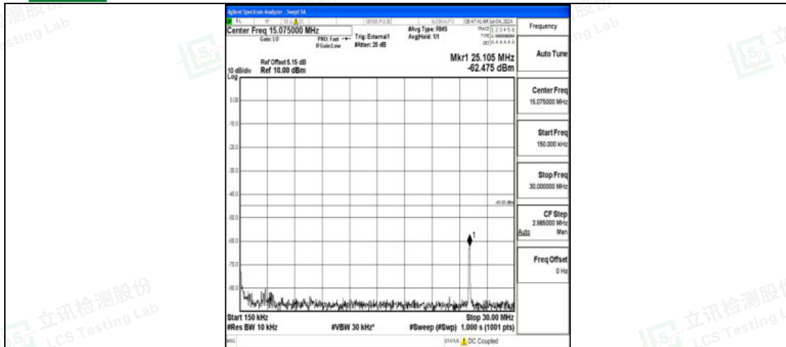
Band41_15MHz_QPSK_40620_1RB#0_0.15~30_0.15~30
