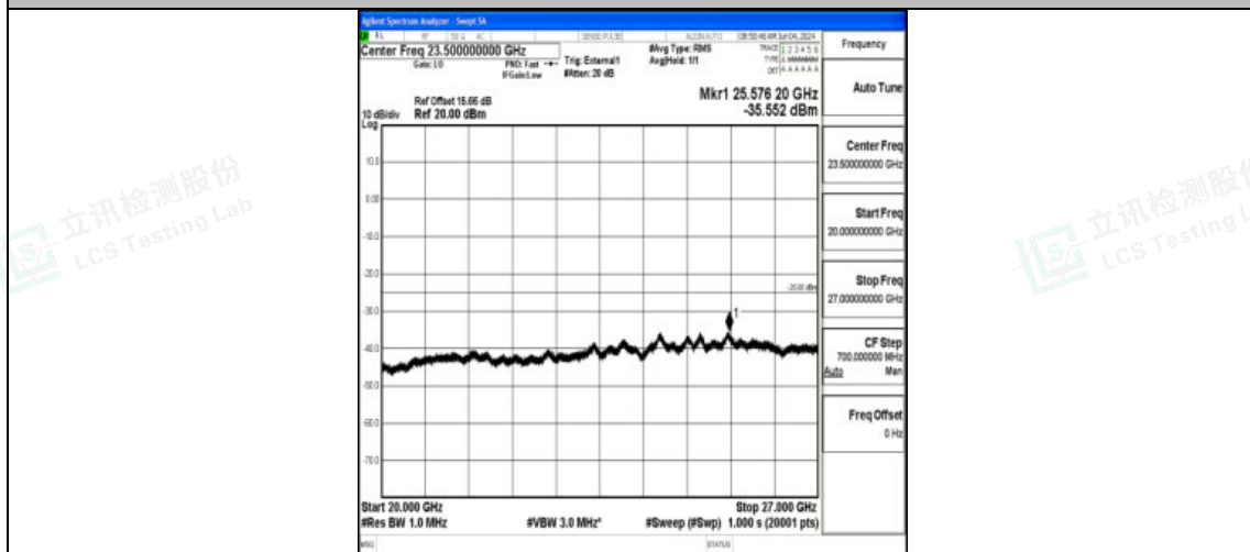
Band41_15MHz_16QAM_40620_1RB#0_20000~27000_20000~27000
