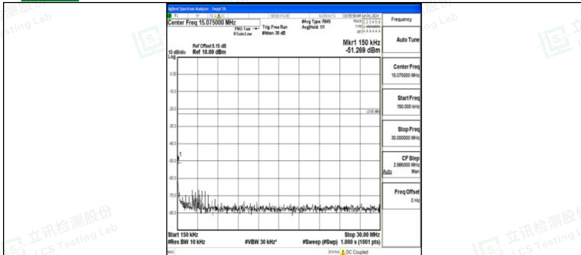
Band17_10MHz_16QAM_23790_1RB#0_0.15~30_0.15~30
