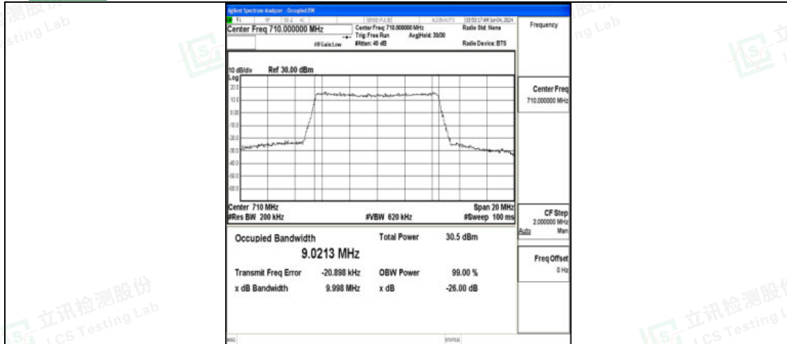
Band17-10MHz-16QAM-23790-50RB#0-PASS
