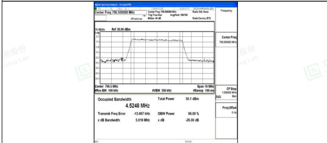
Band17-5MHz-16QAM-23755-25RB#0-PASS
