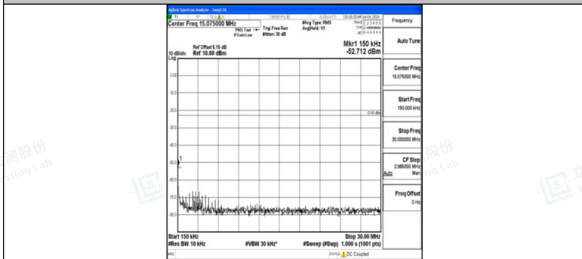
Band12_5MHz_QPSK_23155_1RB#0_0.15~30_0.15~30
