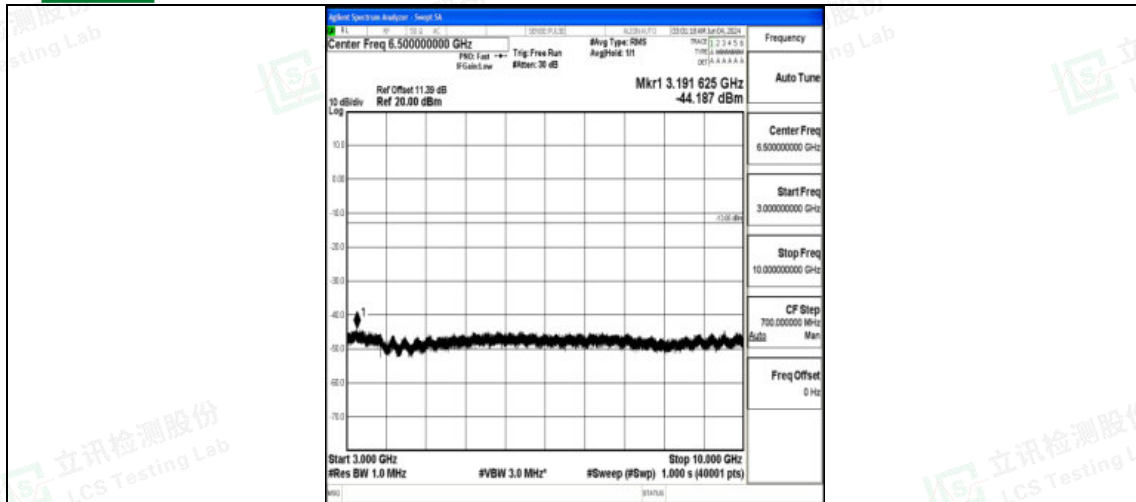
Band12_5MHz_16QAM_23155_1RB#0_3000~10000_3000~10000
