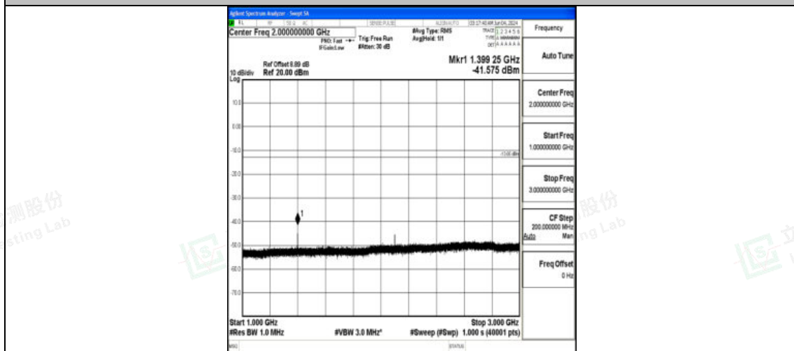
Band12_10MHz_QPSK_23060_1RB#0_1000~3000_1000~3000
