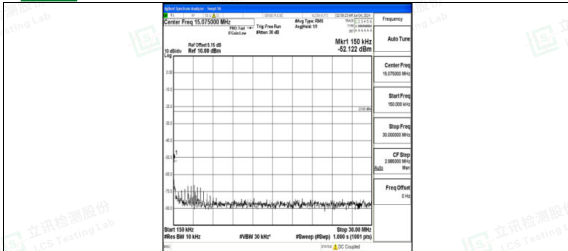
Band12_5MHz_QPSK_23095_1RB#0_0.15~30_0.15~30
