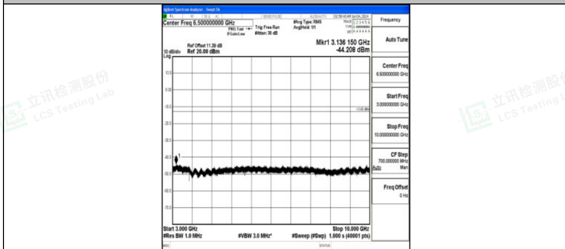
Band12_5MHz_QPSK_23035_1RB#0_3000~10000_3000~10000
