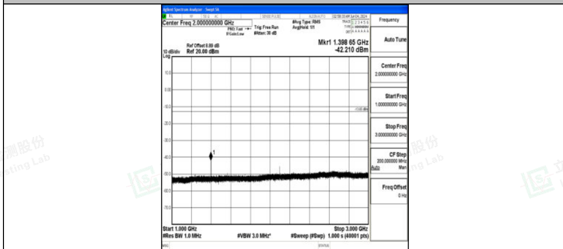
Band12_5MHz_QPSK_23035_1RB#0_1000~3000_1000~3000
