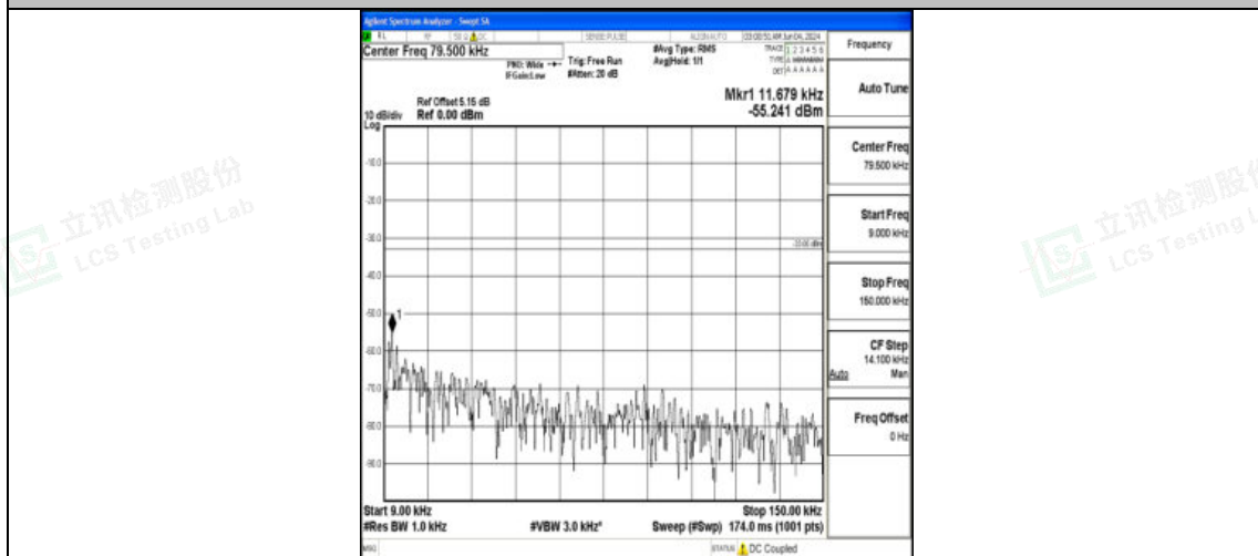
Band12_5MHz_16QAM_23155_1RB#0_0.009-0.15_0.009-0.15
