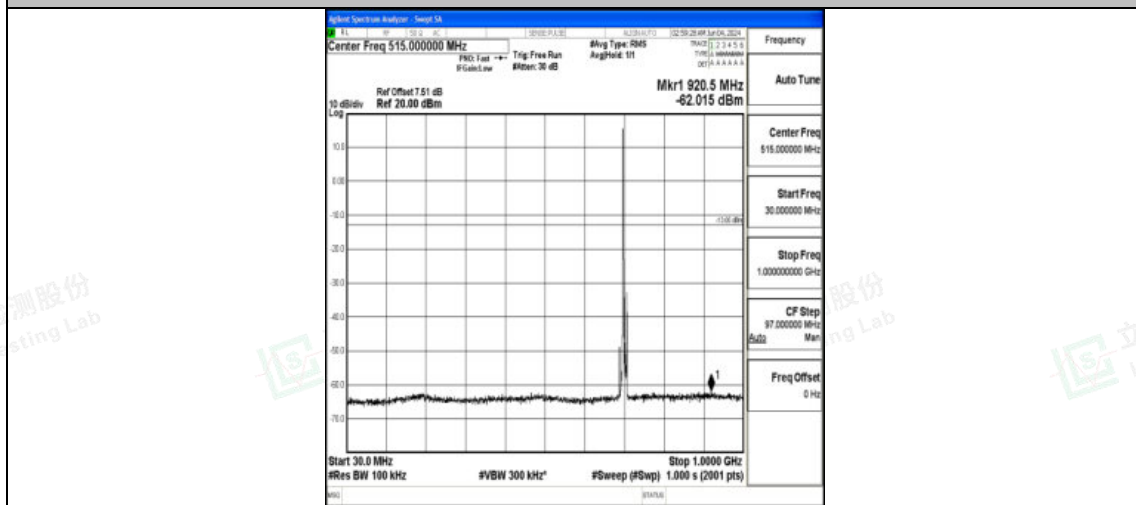
Band12_5MHz_QPSK_23095_1RB#0_30~1000_30~1000
