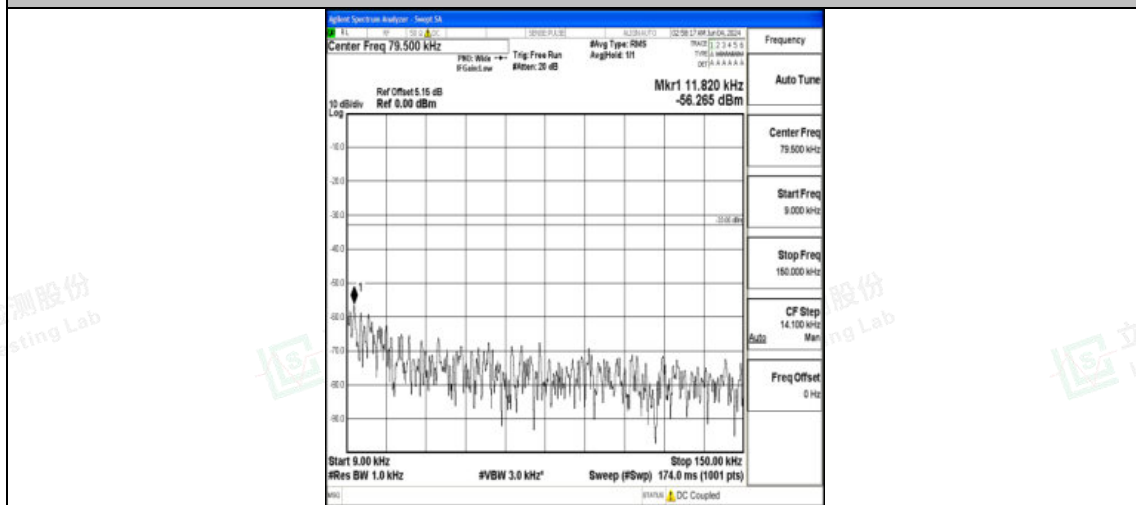
Band12_5MHz_QPSK_23035_1RB#0_0.009~0.15_0.009~0.15
