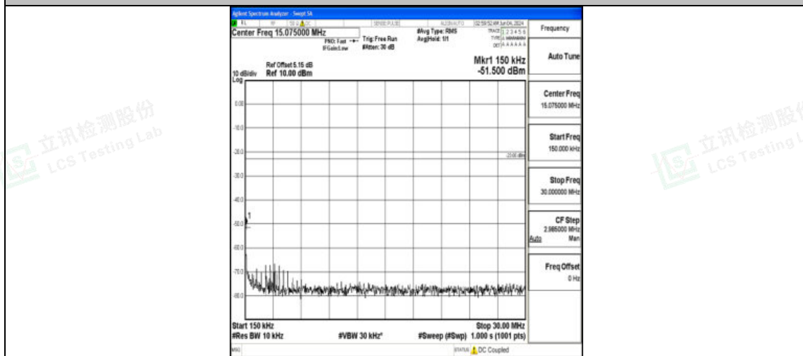
Band12_5MHz_16QAM_23095_1RB#0_0.15~30_0.15~30
