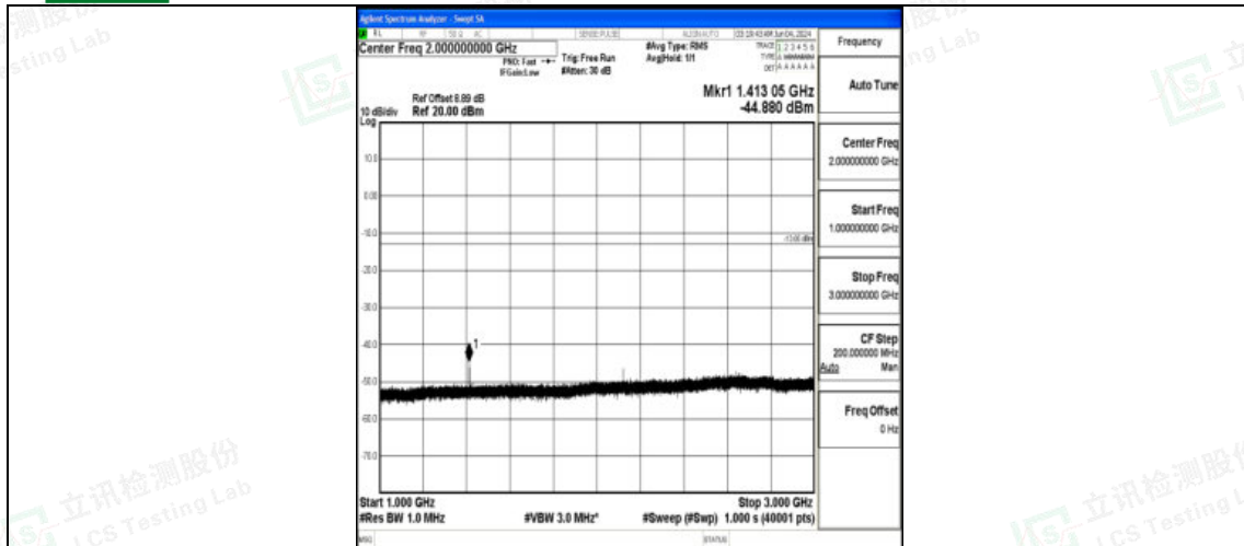
Band12_10MHz_QPSK_23130_1RB#0_1000~3000_1000~3000
