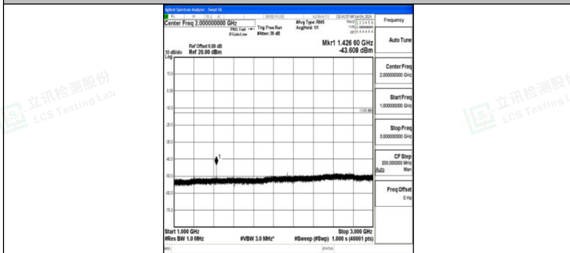
Band12_3MHz_16QAM_23165_1RB#0_1000~3000_1000~3000
