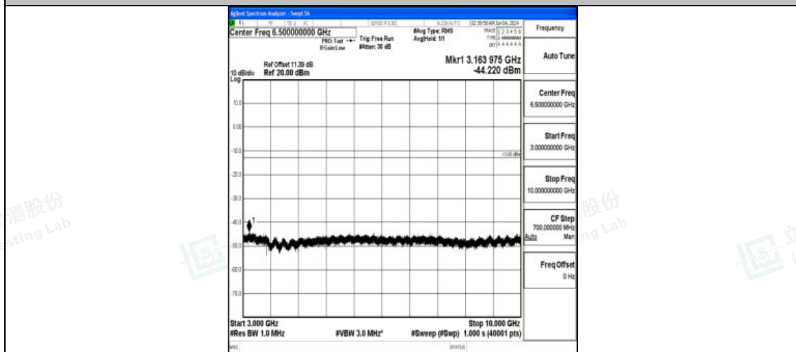
Band12_3MHz_16QAM_23025_1RB#0_3000~10000_3000~10000
