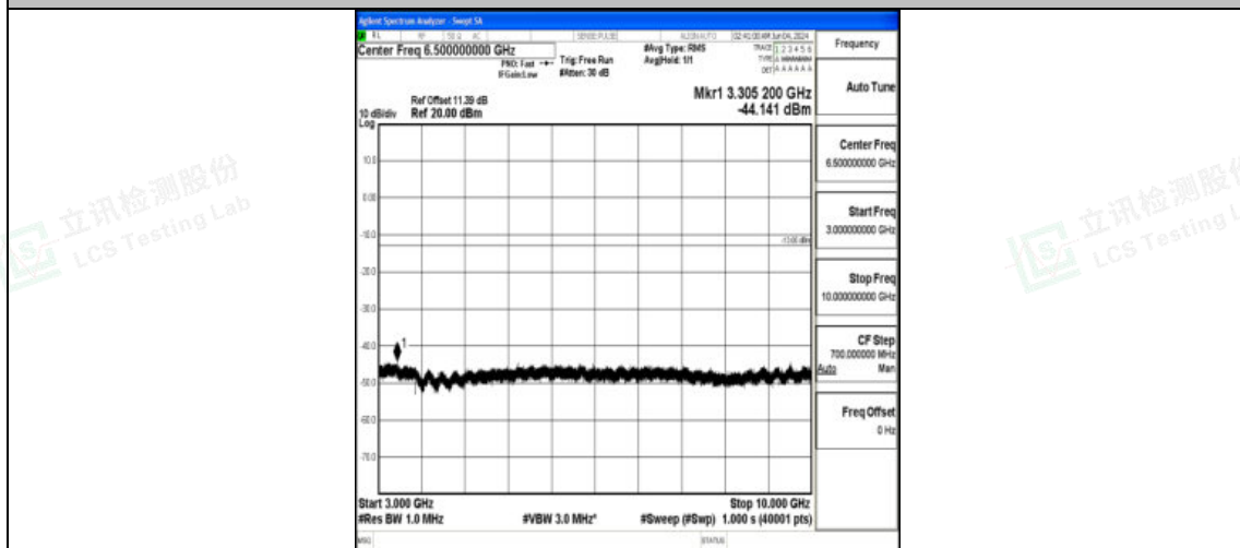
Band12_3MHz_16QAM_23095_1RB#0_3000~10000_3000~10000
