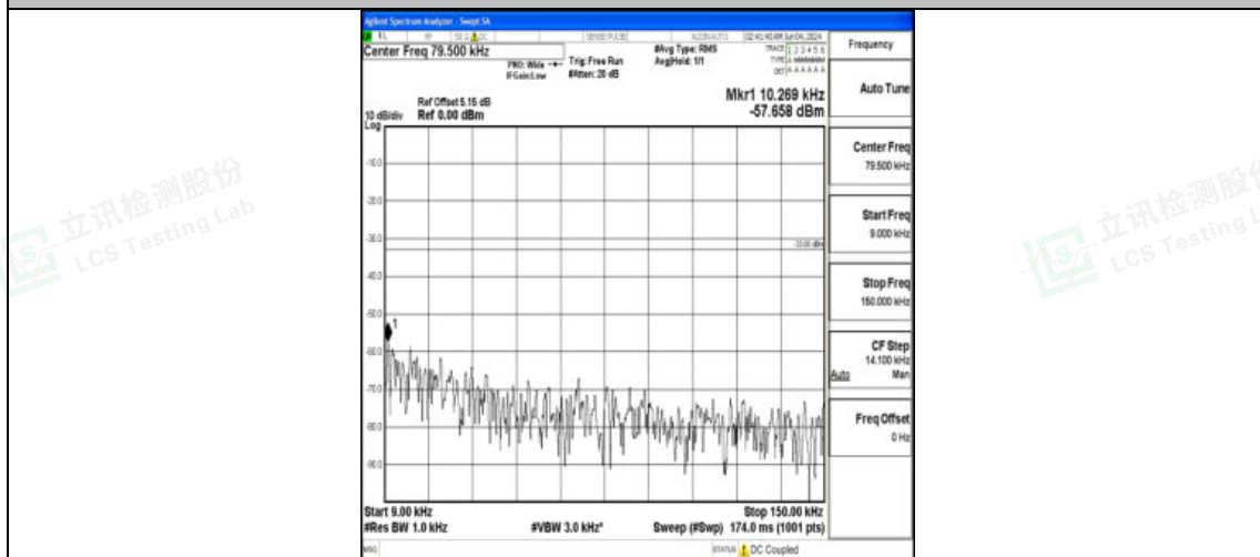
Band12_3MHz_16QAM_23165_1RB#0_0.009-0.15_0.009-0.15
