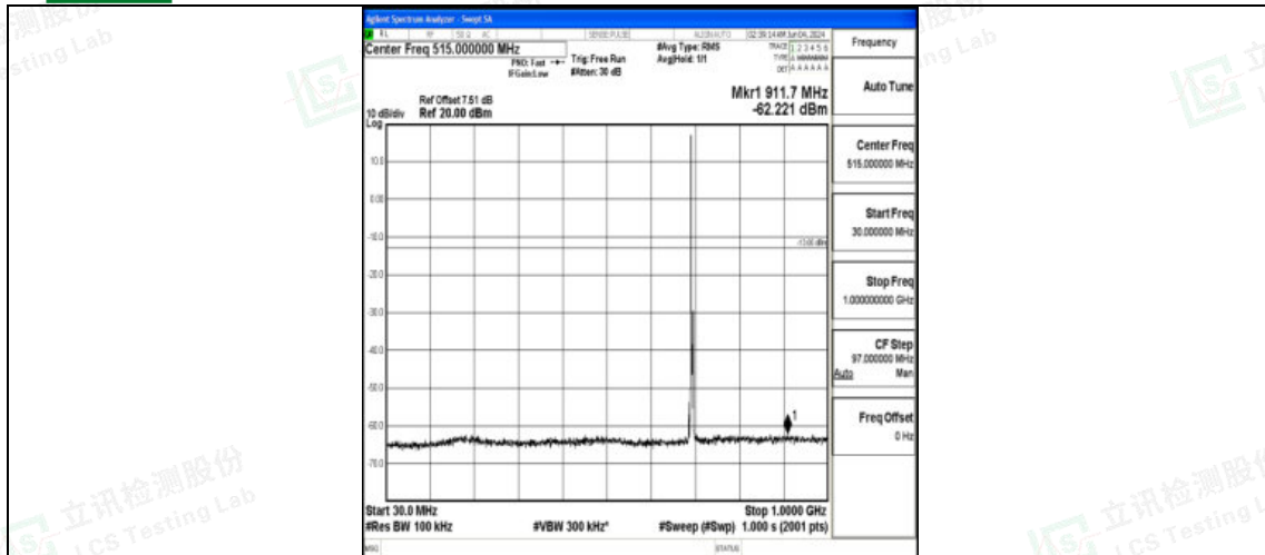
Band12_3MHz_QPSK_23025_1RB#0_30~1000_30~1000
