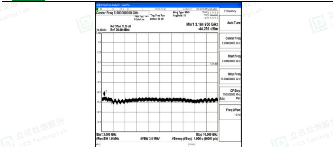
Band12_3MHz_16QAM_23165_1RB#0_3000~10000_3000~10000
