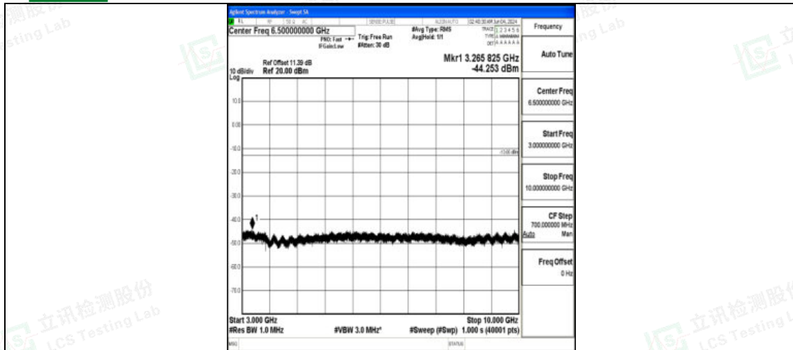
Band12_3MHz_QPSK_23095_1RB#0_3000-10000_3000-10000
