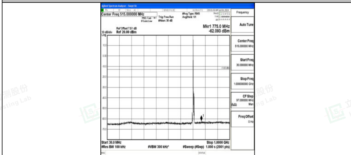
Band12_5MHz_16QAM_23155_1RB#0_30~1000_30~1000
