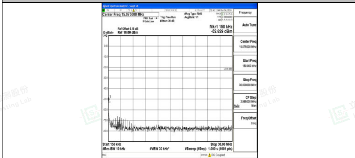
Band12_3MHz_QPSK_23165_1RB#0_0.15~30_0.15~30
