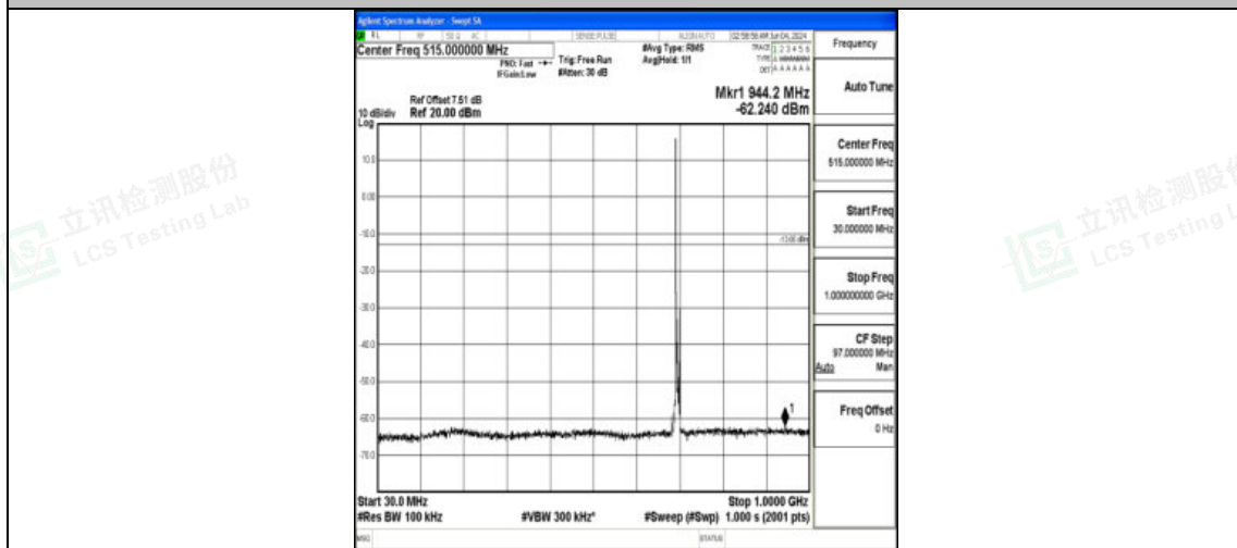
Band12_5MHz_16QAM_23035_1RB#0_30~1000_30~1000
