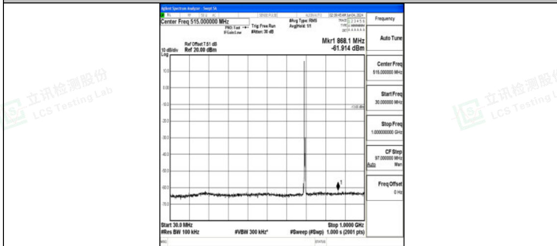
Band12_3MHz_16QAM_23025_1RB#0_30~1000_30~1000
