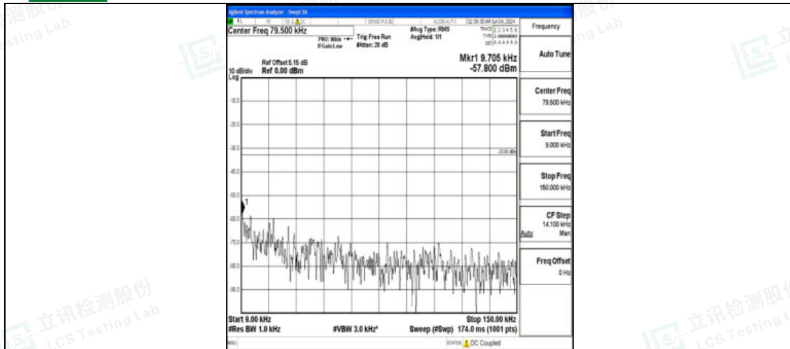
Band12_3MHz_16QAM_23025_1RB#0_0.009~0.15_0.009~0.15
