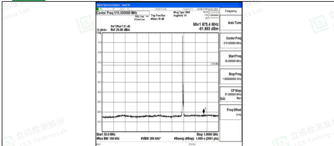
Band12_5MHz_QPSK_23035_1RB#0_30~1000_30~1000
