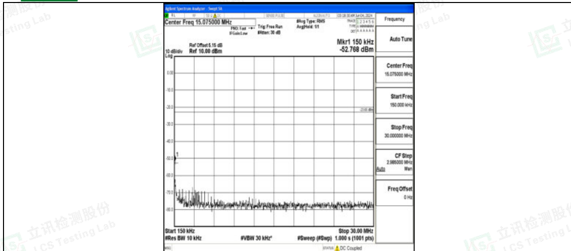
Band12_10MHz_QPSK_23095_1RB#0_0.15-30_0.15-30
