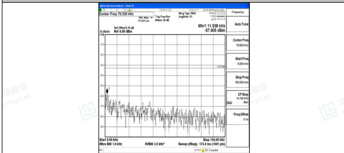
Band12_3MHz_16QAM_23095_1RB#0_0.009-0.15_0.009-0.15
