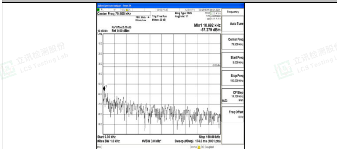
Band12_10MHz_16QAM_23130_1RB#0_0.009~0.15_0.009~0.15
