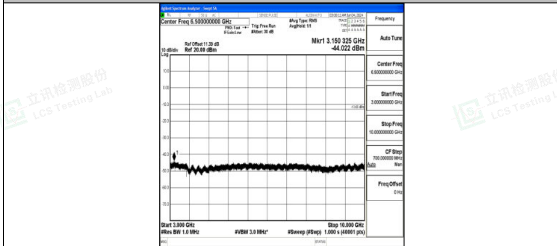
Band12_5MHz_16QAM_23095_1RB#0_3000~10000_3000~10000
