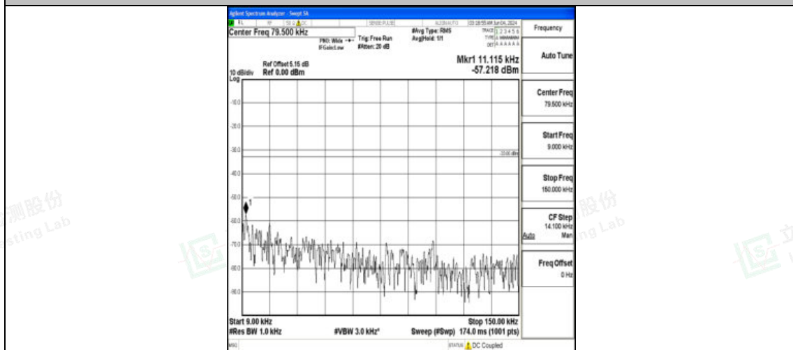
Band12_10MHz_16QAM_23095_1RB#0_0.009~0.15_0.009~0.15
