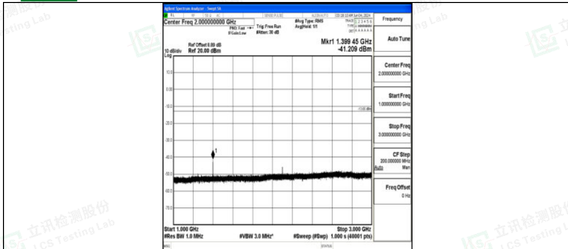
Band12_10MHz_16QAM_23060_1RB#0_1000~3000_1000~3000
