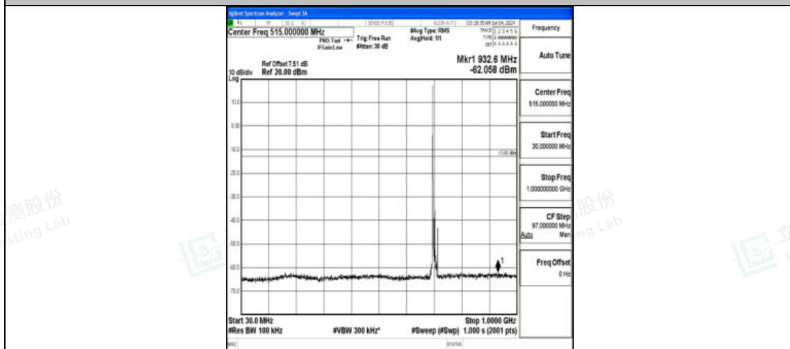
Band12_10MHz_QPSK_23095_1RB#0_30-1000_30-1000
