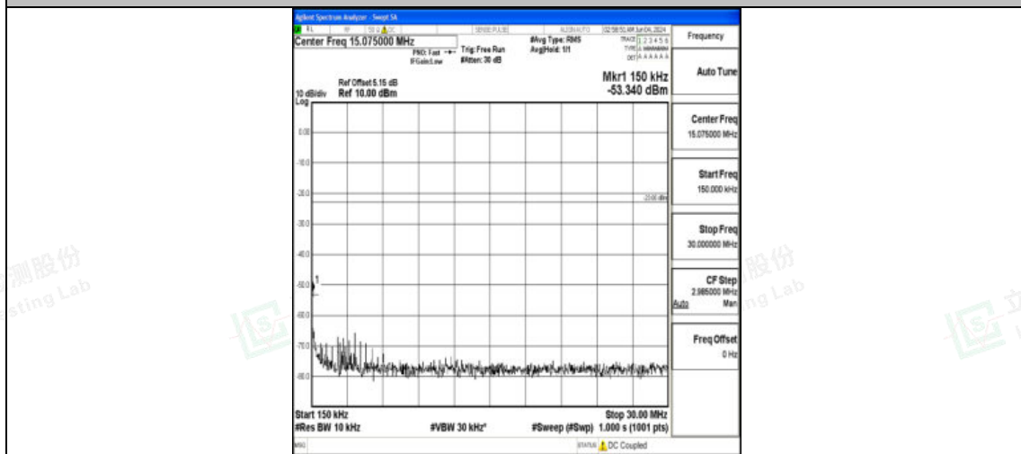
Band12_5MHz_16QAM_23035_1RB#0_0.15~30_0.15~30
