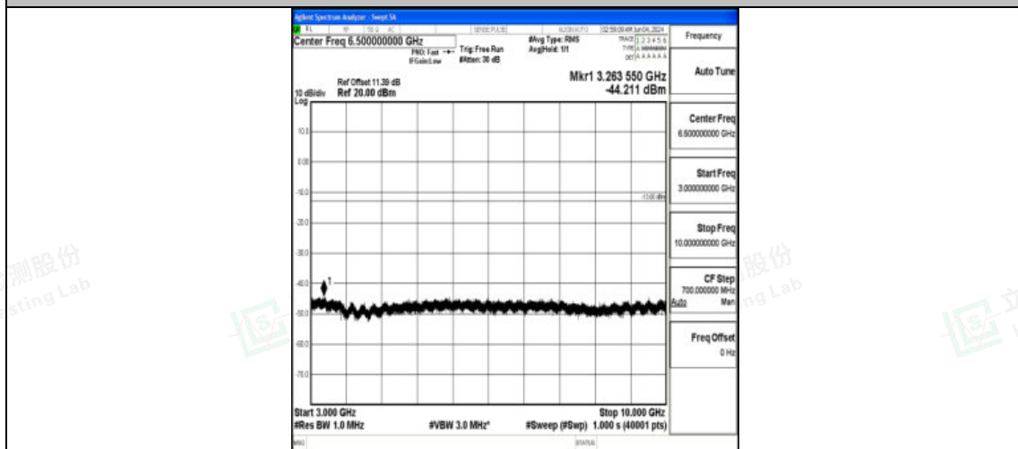
Band12_5MHz_16QAM_23035_1RB#0_3000~10000_3000~10000
