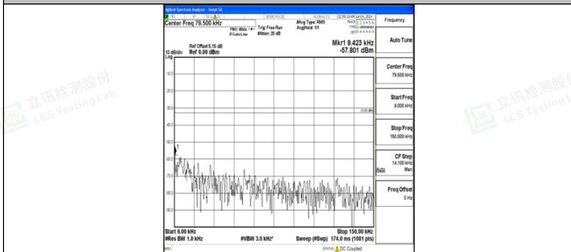
Band12_5MHz_QPSK_23095_1RB#0_0.009~0.15_0.009~0.15
