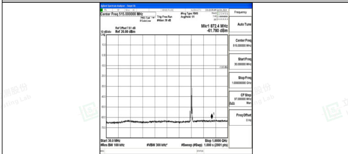
Band12_10MHz_16QAM_23130_1RB#0_30~1000_30~1000
