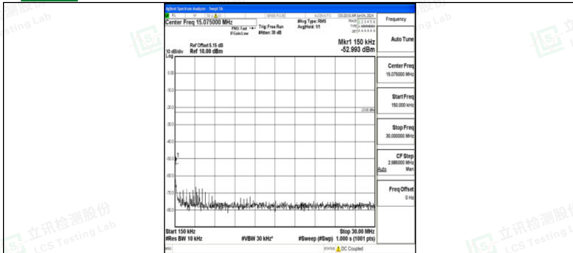
Band12_10MHz_16QAM_23130_1RB#0_0.15~30_0.15~30
