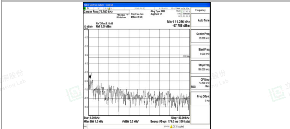
Band12_10MHz_QPSK_23060_1RB#0_0.009~0.15_0.009~0.15
