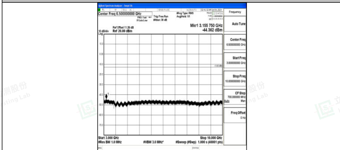
Band12_3MHz_QPSK_23165_1RB#0_3000-10000_3000-10000
