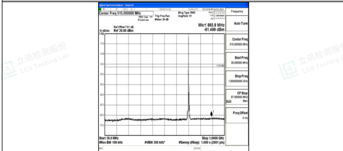
Band12_10MHz_QPSK_23130_1RB#0_30~1000_30~1000
