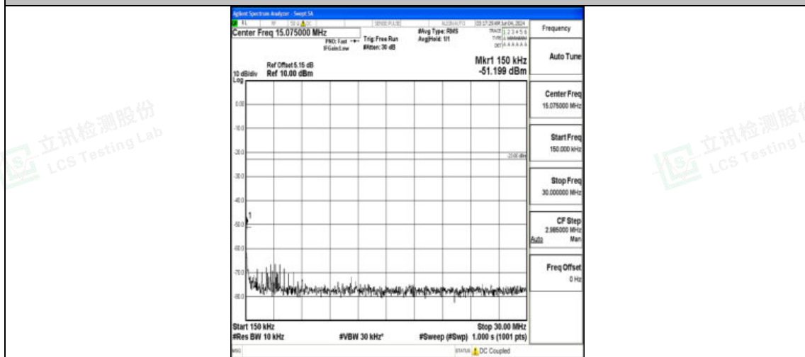
Band12_10MHz_QPSK_23060_1RB#0_0.15~30_0.15~30
