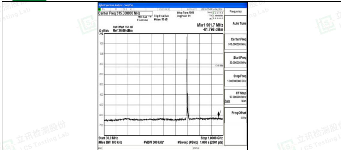
Band12_10MHz_16QAM_23095_1RB#0_30~1000_30~1000
