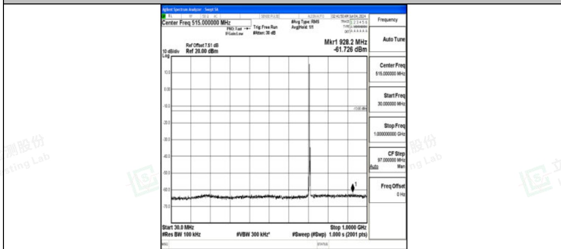
Band12_3MHz_16QAM_23165_1RB#0_30~1000_30~1000
