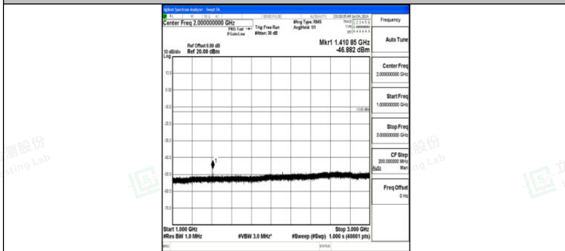
Band12_5MHz_16QAM_23095_1RB#0_1000~3000_1000~3000
