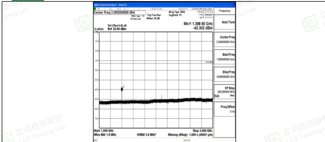
Band12_5MHz_16QAM_23035_1RB#0_1000~3000_1000~3000
