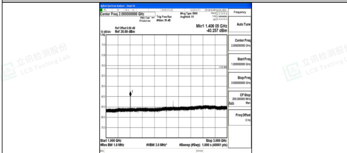
Band12_10MHz_QPSK_23095_1RB#0_1000-3000_1000-3000
