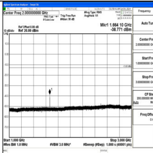
Band5_10MHz_QPSK_20525_1RB#0_1000~3000_1000~3000
