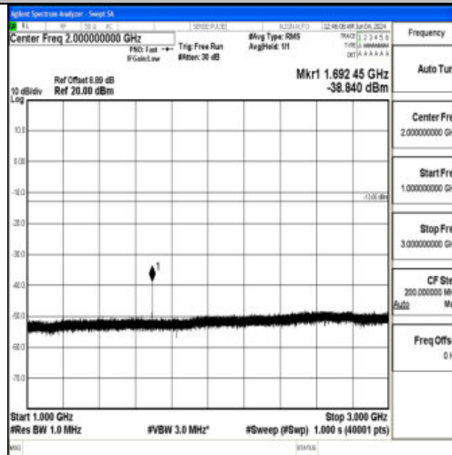
Band5_3MHz_16QAM_20635_1RB#0_1000~3000_1000~3000
