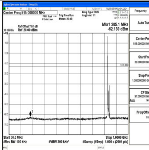
Band5_10MHz_QPSK_20525_1RB#0_30~1000_30~1000
