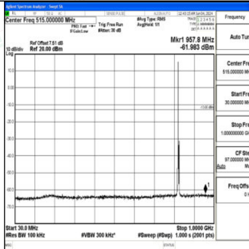
Band5_3MHz_QPSK_20415_1RB#0_30~1000_30~1000
