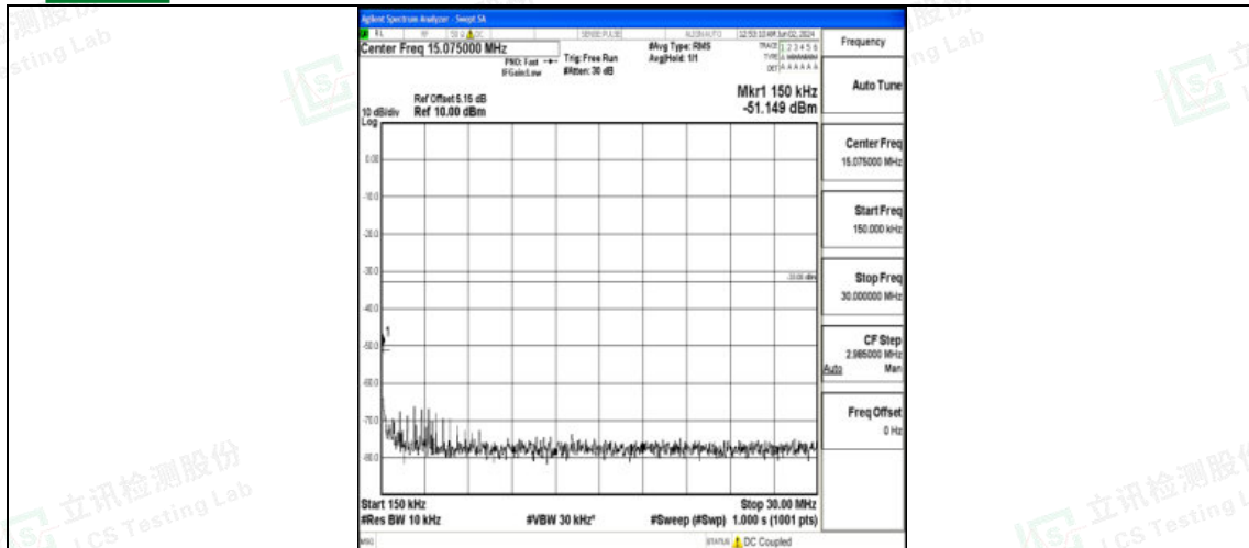
Band2_3MHz_16QAM_18900_1RB#0_0.15~30_0.15~30
