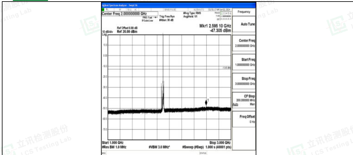
Band2_15MHz_16QAM_19125_1RB#0_1000~3000_1000~3000
