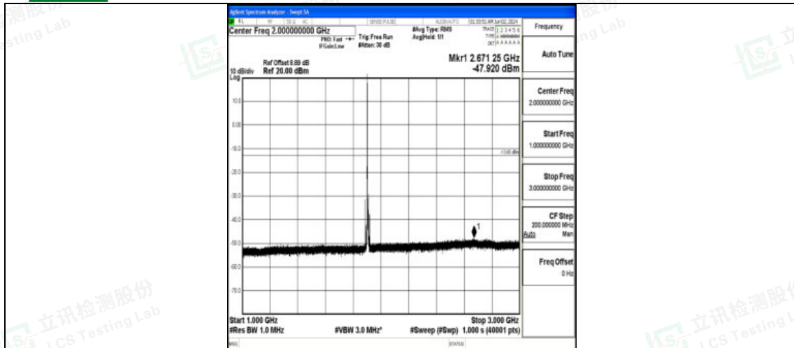
Band2_10MHz_16QAM_19150_1RB#0_1000~3000_1000~3000
