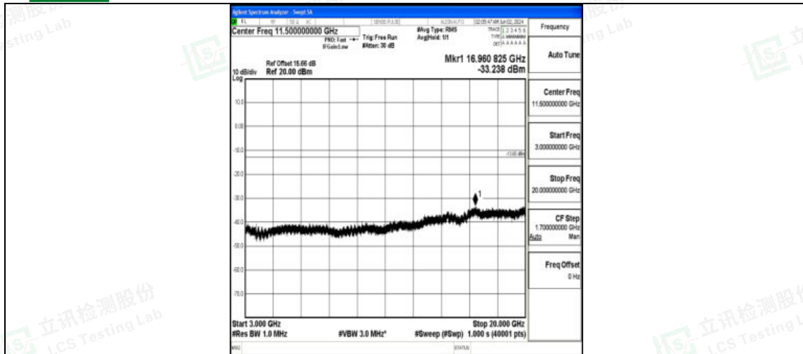
Band2_20MHz_QPSK_18700_1RB#0_3000-20000_3000-20000
