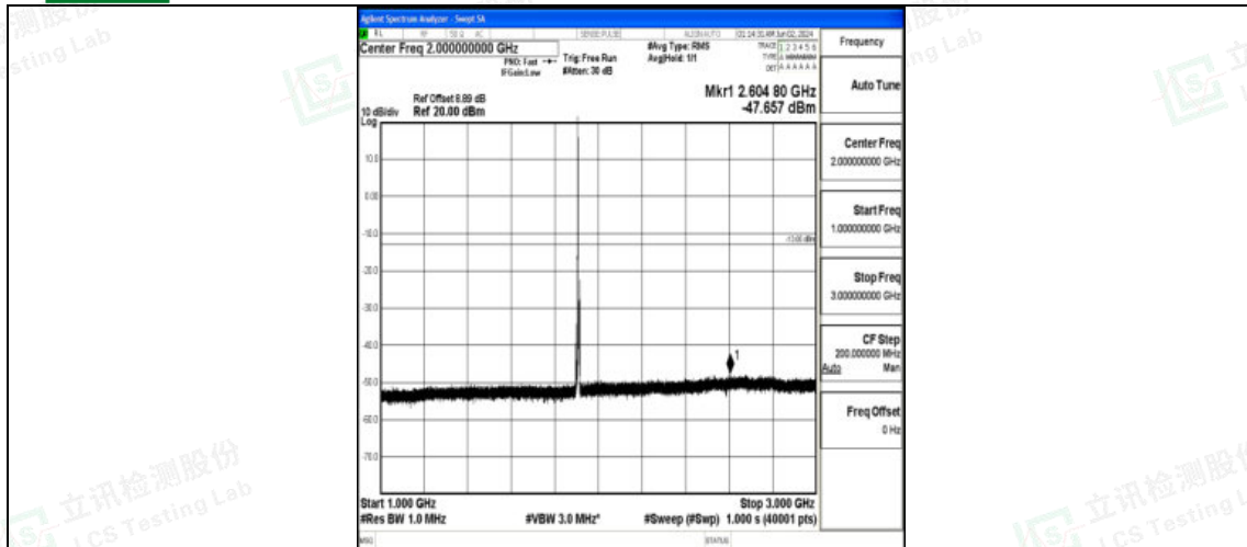
Band2_5MHz_16QAM_19175_1RB#0_1000~3000_1000~3000
