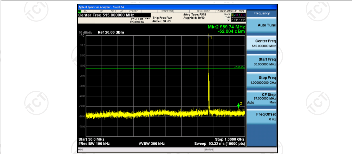
Band13-5MHz-16QAM-23205-1RB#0-Range1:30~1000MHz
