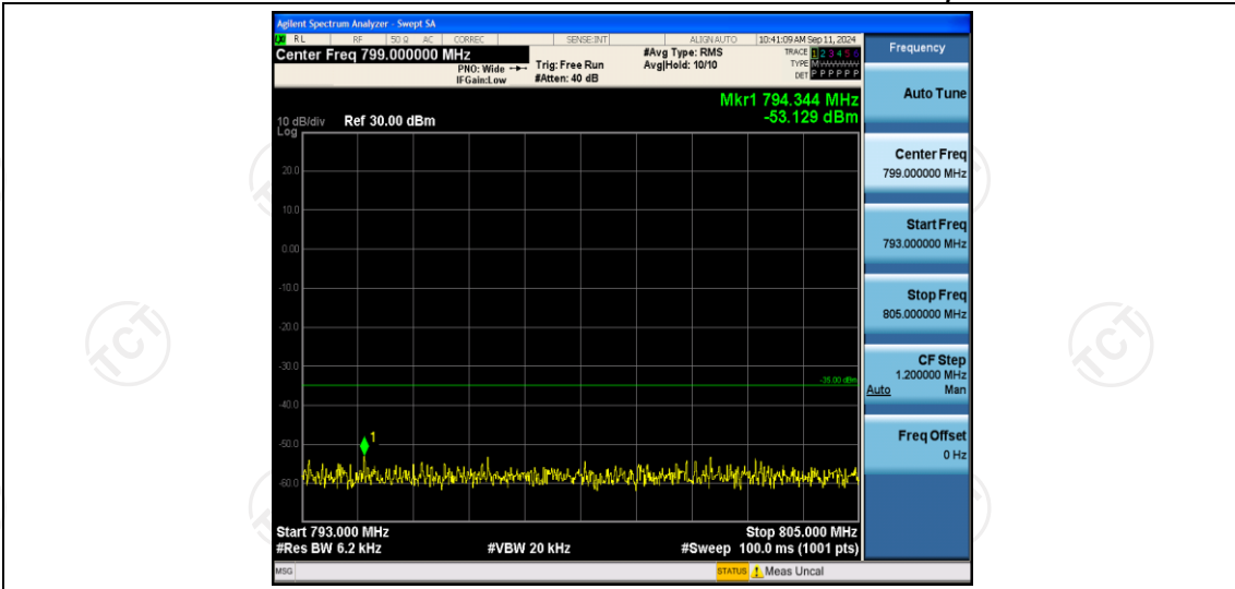
Band13-5MHz-16QAM-23205-1RB#0-Range4:793~805MHz
