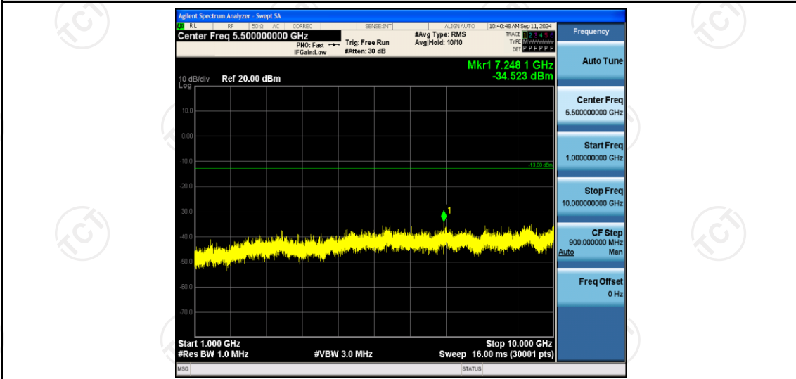
Band13-5MHz-16QAM-23205-1RB#0-Range2:1000~10000MHz
