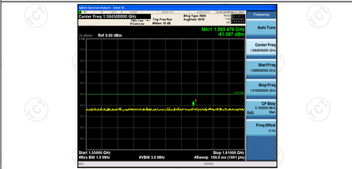
Band13-5MHz-QPSK-23205-1RB#0-Range5:1559~1610MHz
