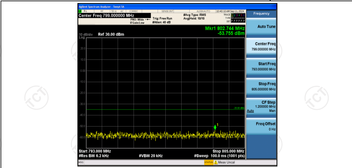
Band13-5MHz-QPSK-23205-1RB#0-Range4:793~805MHz
