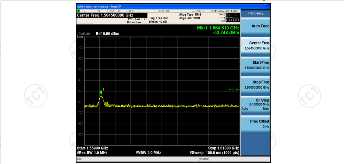
Band13-5MHz-QPSK-23255-1RB#0-Range5:1559~1610MHz
