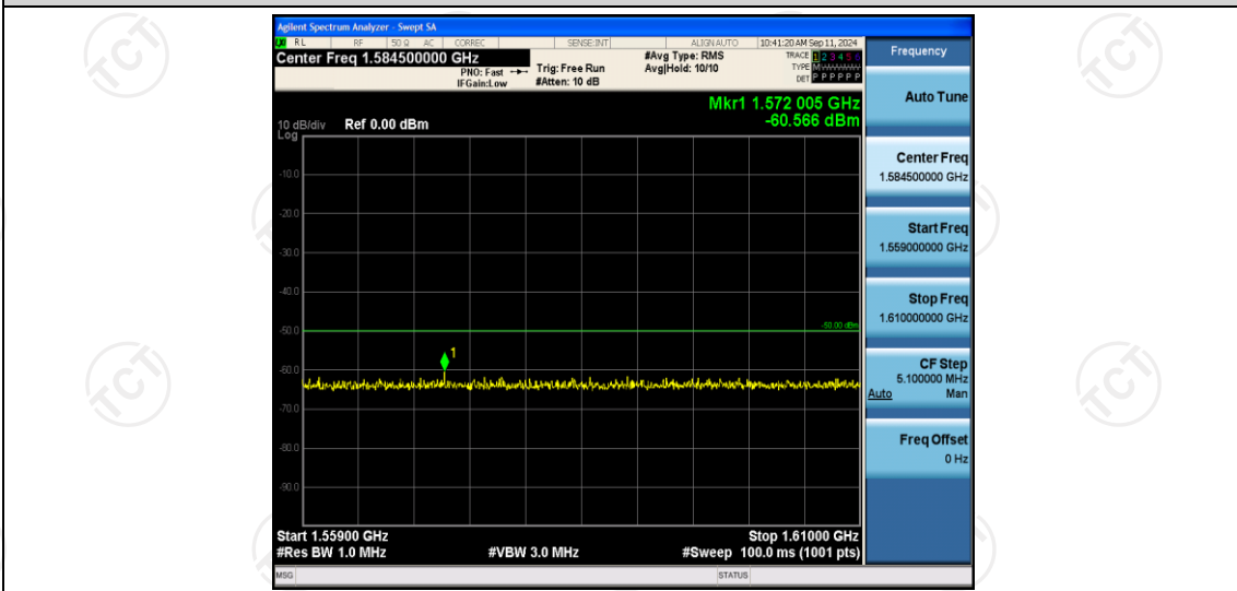
Band13-5MHz-16QAM-23205-1RB#0-Range5:1559~1610MHz
