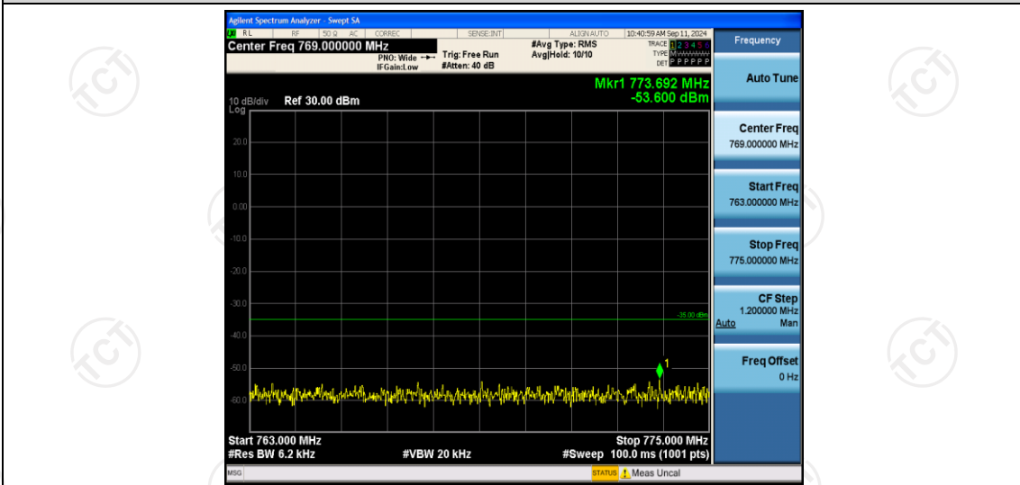
Band13-5MHz-16QAM-23205-1RB#0-Range3:763~775MHz
