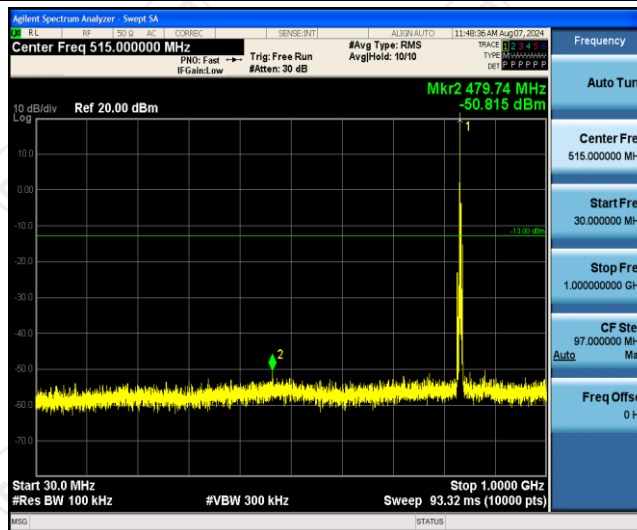
Band5-3MHz-16QAM-20525-1RB#0-Range1:30~1000MHz
