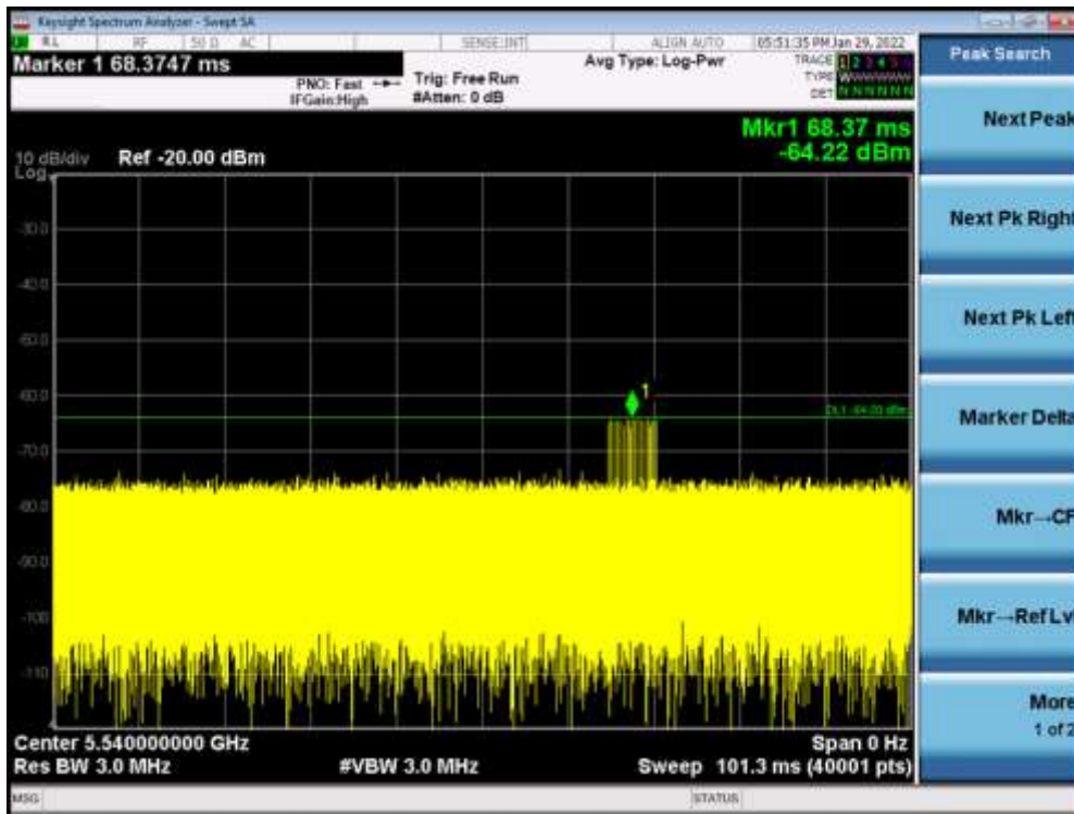
Radar Signal 3
