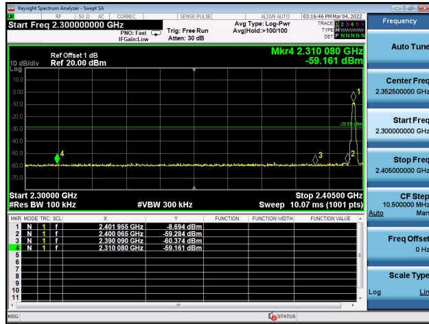
Left bandedge
