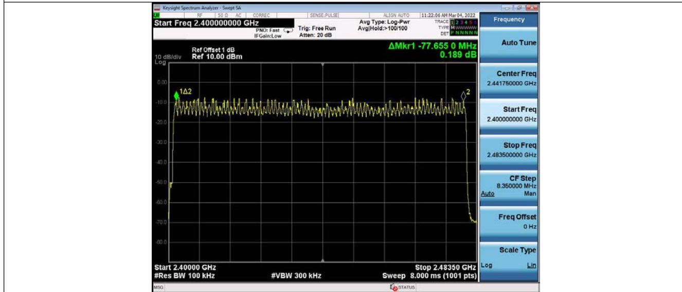
π/4DQPSK Modulation
