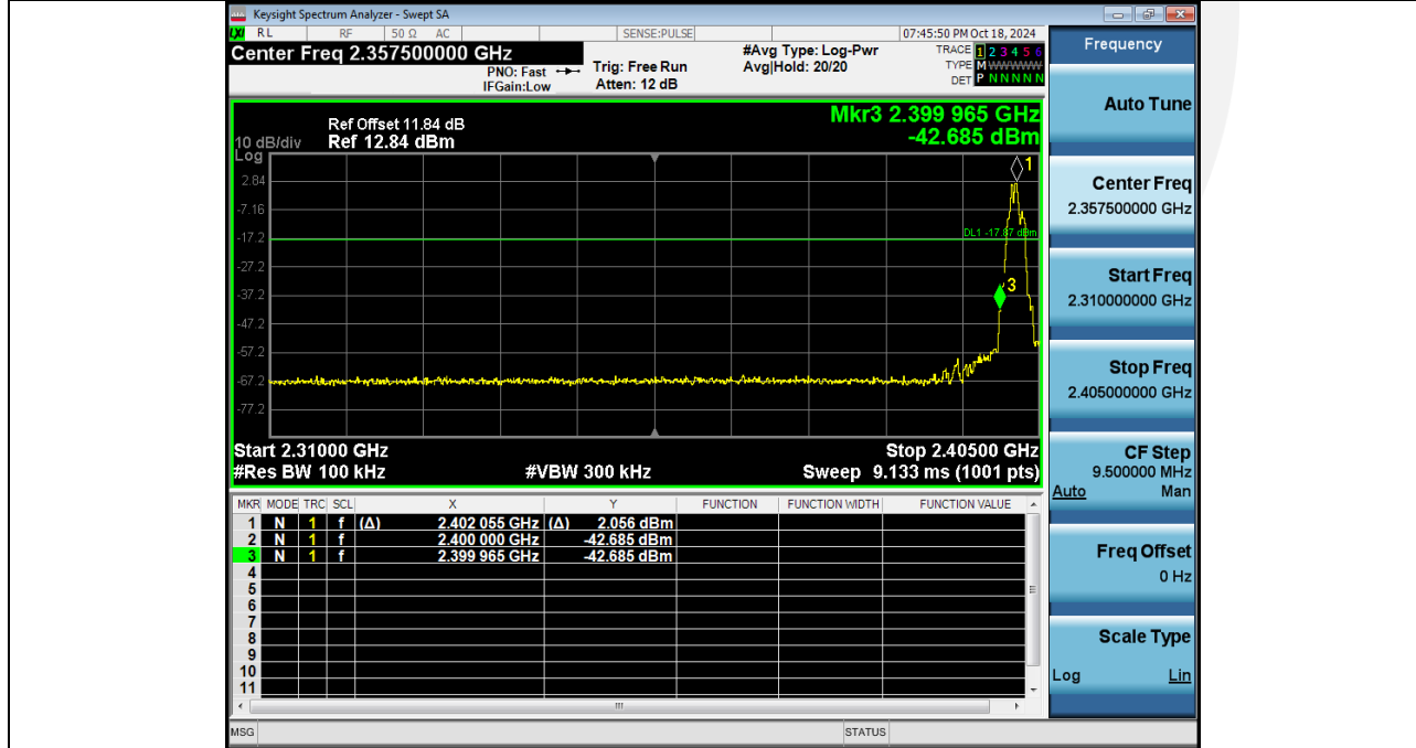
2 Bandedge_NVNT_ANT1_2Mbps_2402
