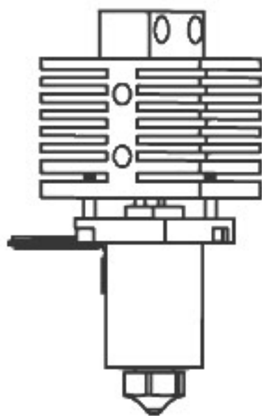
Ordinary Hotend
