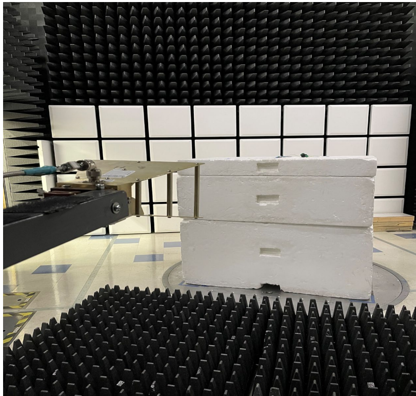
RF Radiated 1-18 GHz
