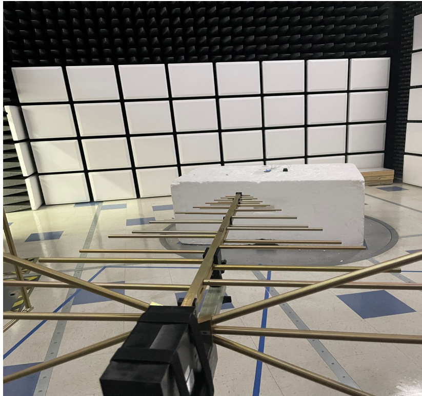
RF Radiated 30 MHz-1GHz
