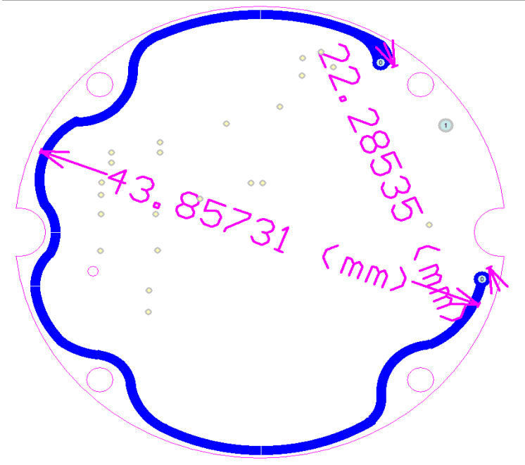
AntennaPhoto&Length(mm)
