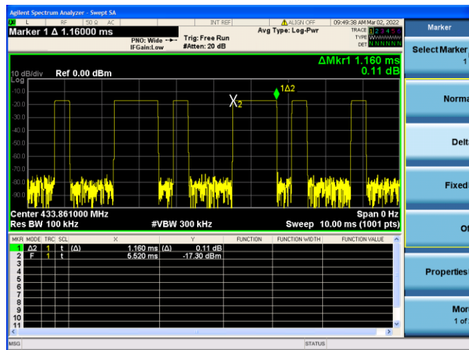
(Time per burst: 1.160ms*18pcs)
