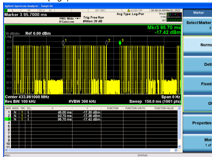
(Transmit cycle 50.70ms)
