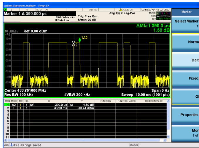
(Time per burst: 0.390ms*7pcs)
