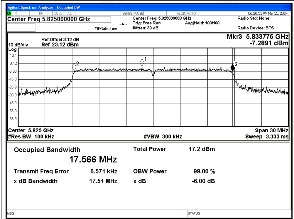
-6dB Bandwidth NVNT n20 5825MHz Ant
