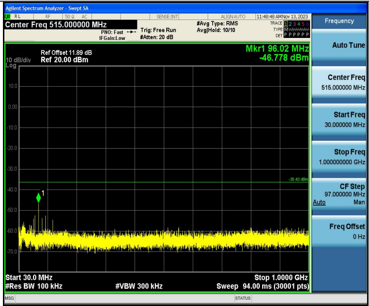
BLE_1M-Ant1-2402-30~1000-PASS
