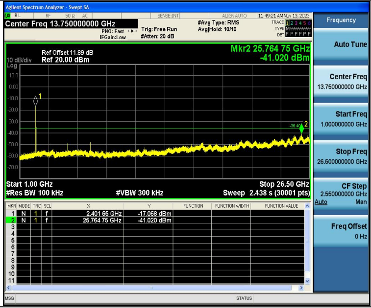
BLE_1M-Ant1-2402-1000~26500-PASS
