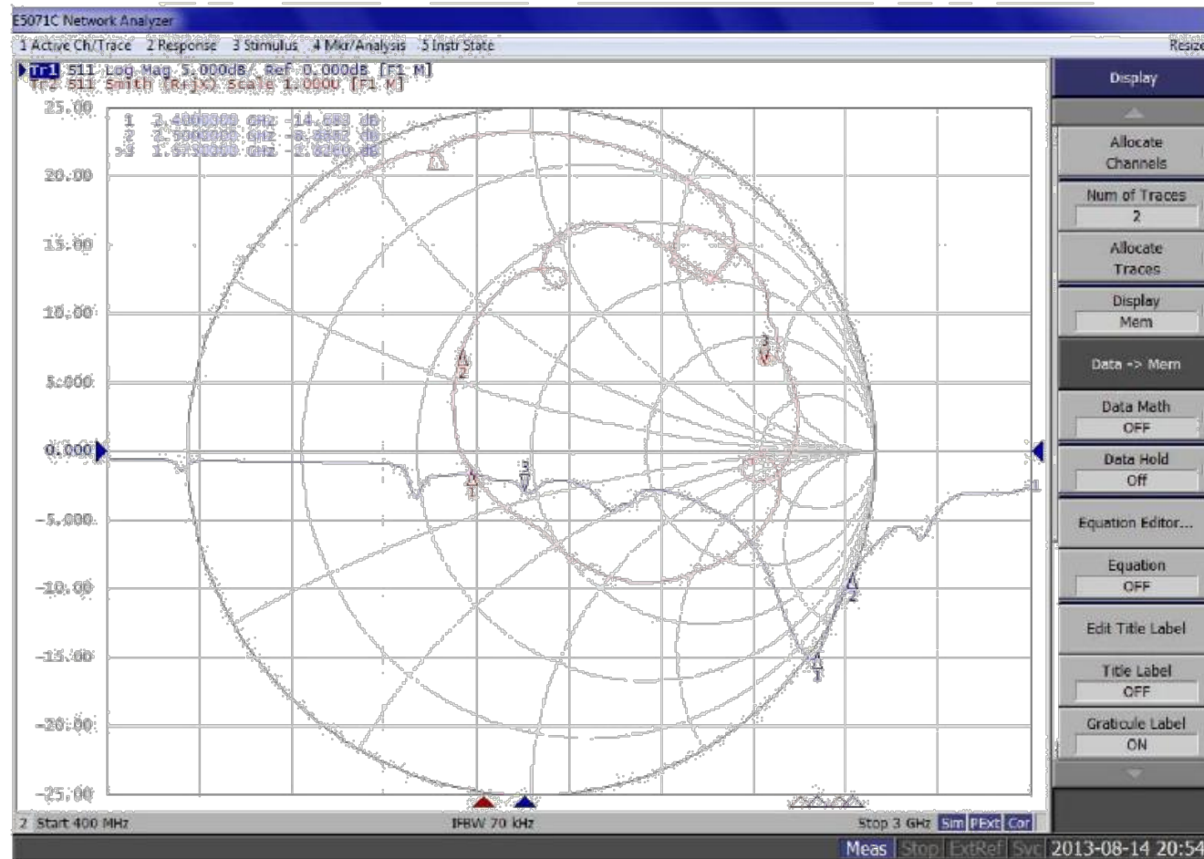
2.4G BT: Main line matches 0 ohm
