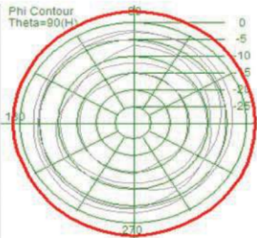
Peak Gain: 2.87dBi
