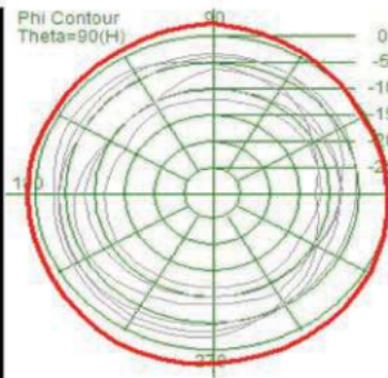
Peak Gain: 3.02dBi
