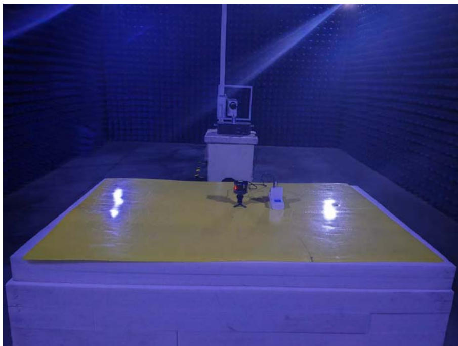
Photo of Radiated Emission Measurement Below 30MHz
