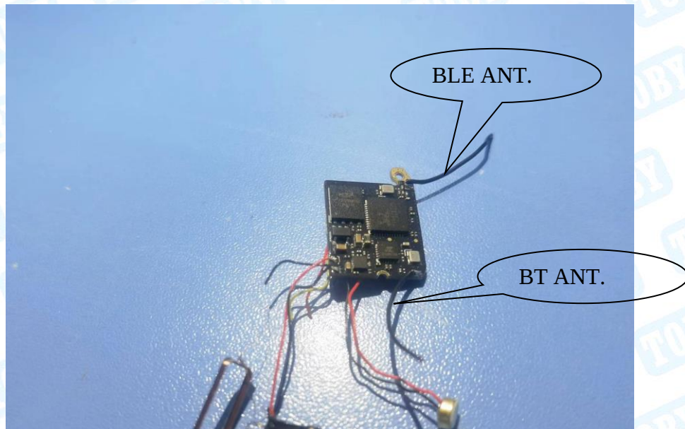
Photo 11 Appearance of PCB
