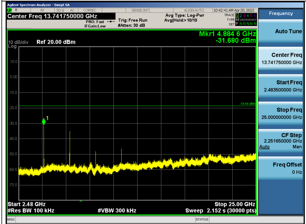
Test_Graph_LE1M_ANT1_2445_1Mbps_Higher Band Emissions
