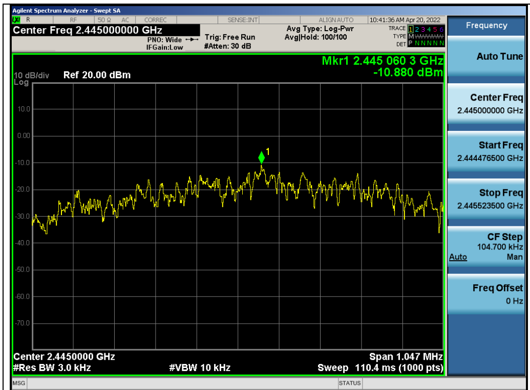
Test_Graph_LE1M_ANT1_2445_1Mbps_PSD
