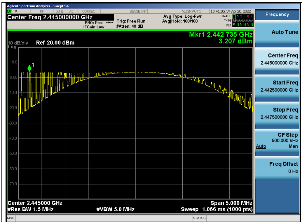
Test_Graph_LE1M_ANT1_2445_1Mbps_Peak Power
