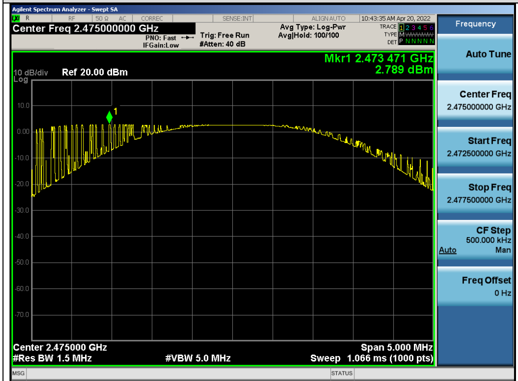
Test_Graph_LE1M_ANT1_2475_1Mbps_Peak Power
