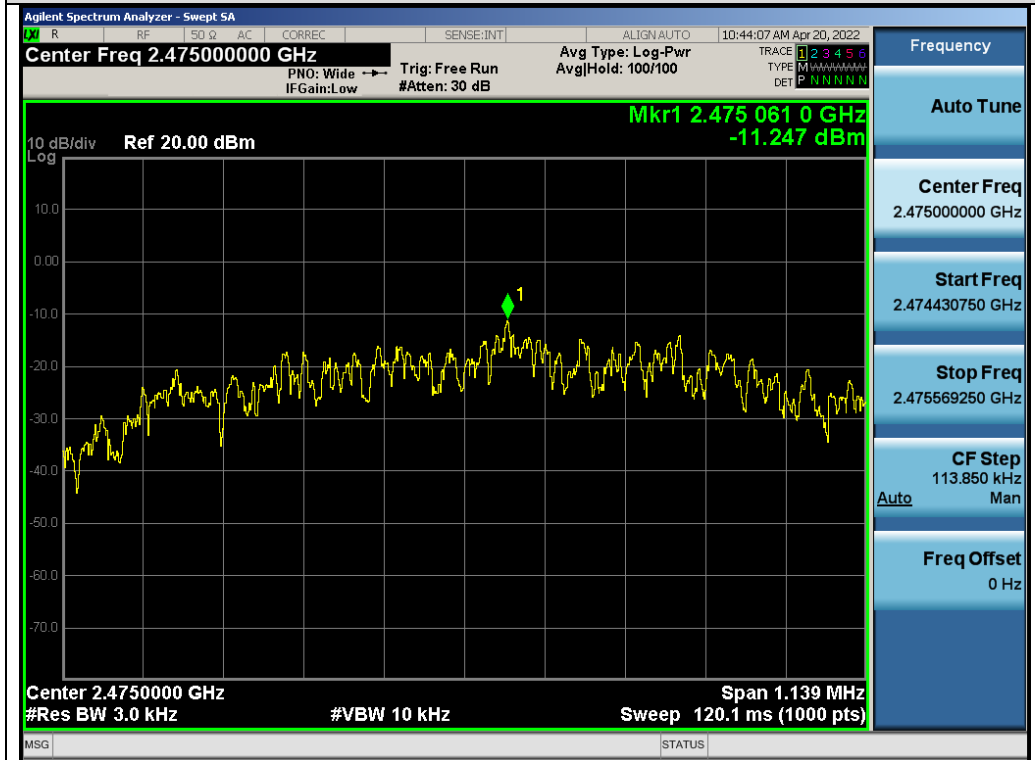
Test_Graph_LE1M_ANT1_2475_1Mbps_PSD
