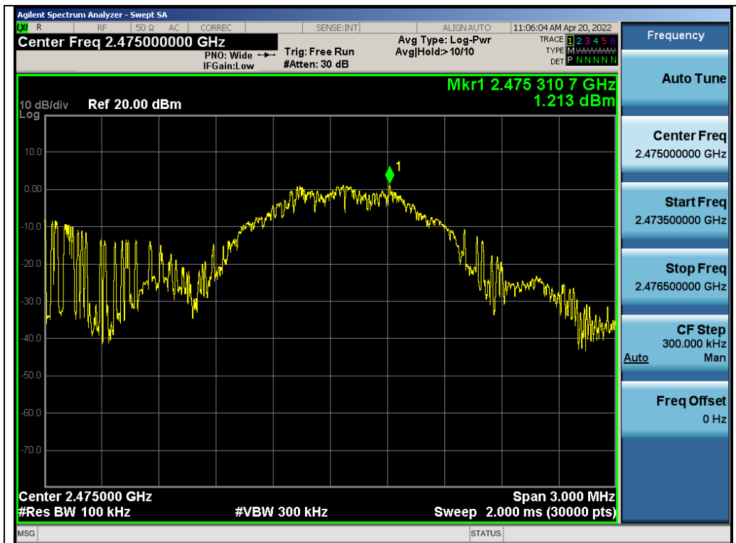
Test_Graph_LE1M_ANT1_2475_1Mbps_Reference Level
