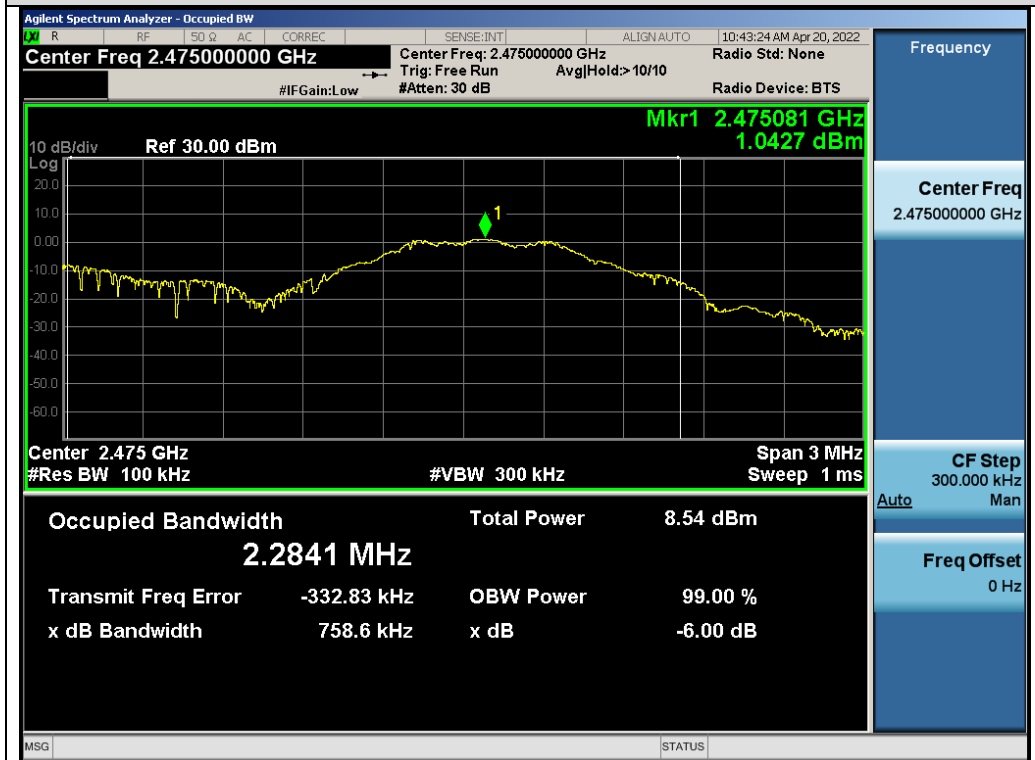
Test_Graph_LE1M_ANT1_2475_1Mbps_DTSBW
