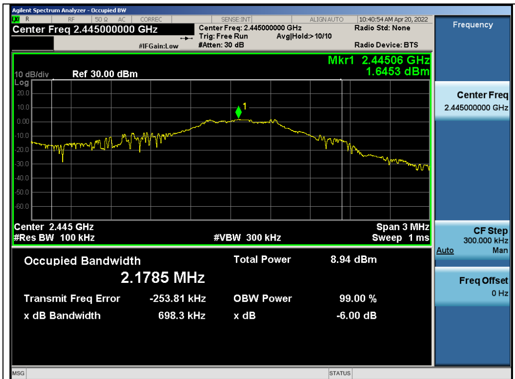
Test_Graph_LE1M_ANT1_2445_1Mbps_DTSBW
