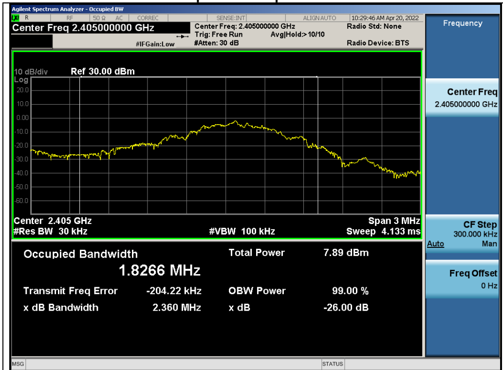
Test_Graph_LE1M_ANT1_2405_1Mbps_OBW
