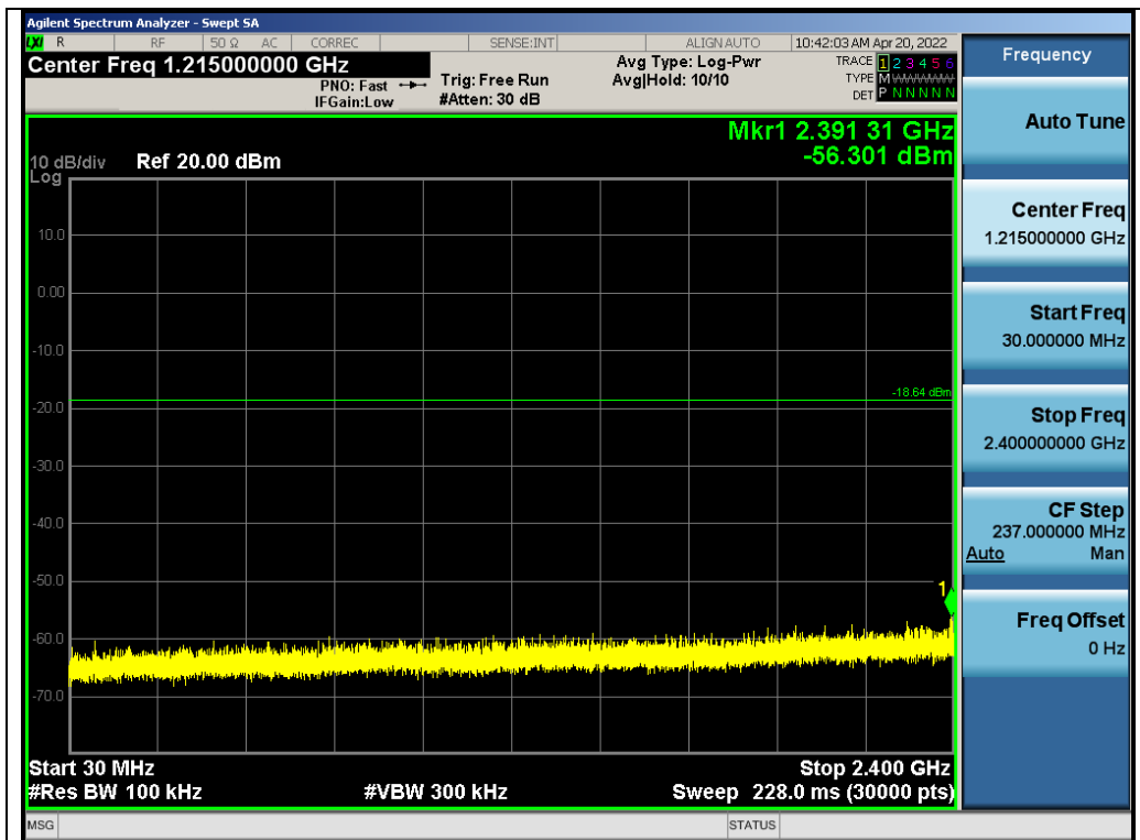
Test_Graph_LE1M_ANT1_2445_1Mbps_Lower Band Emissions
