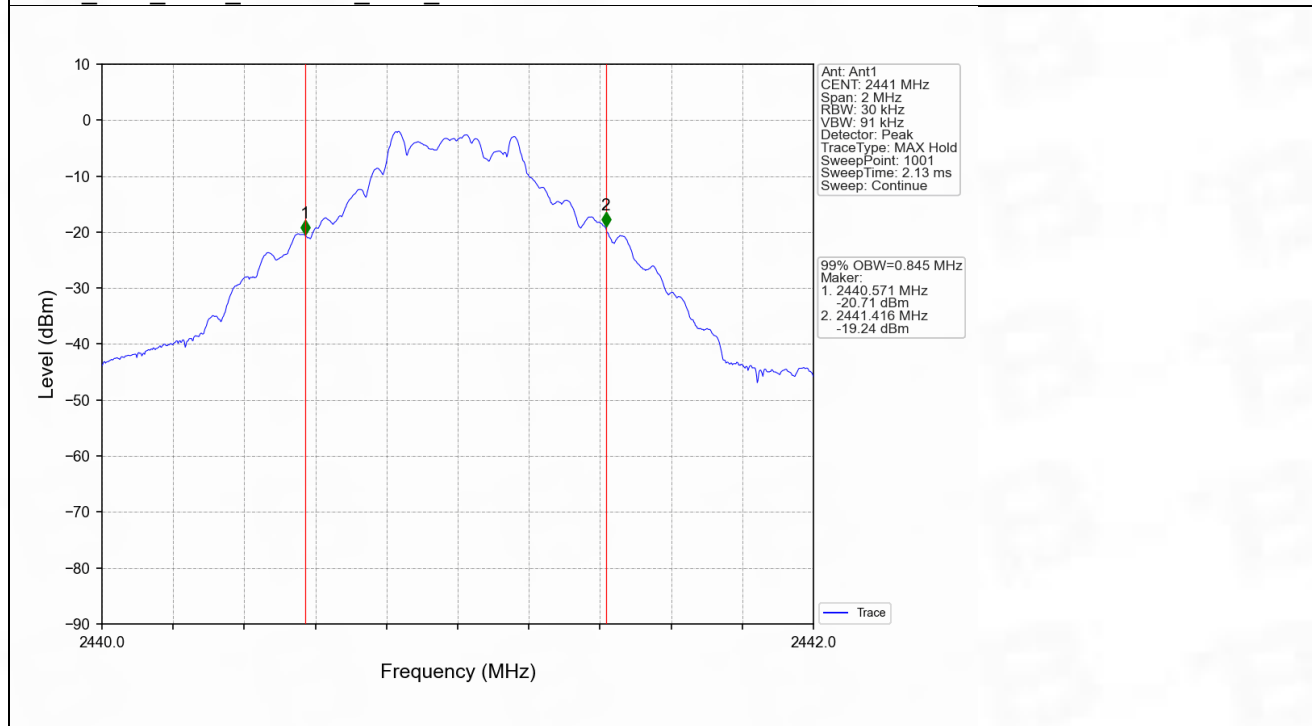
GFSK_DH5_MCH_2441MHz_Ant1_NTNV
