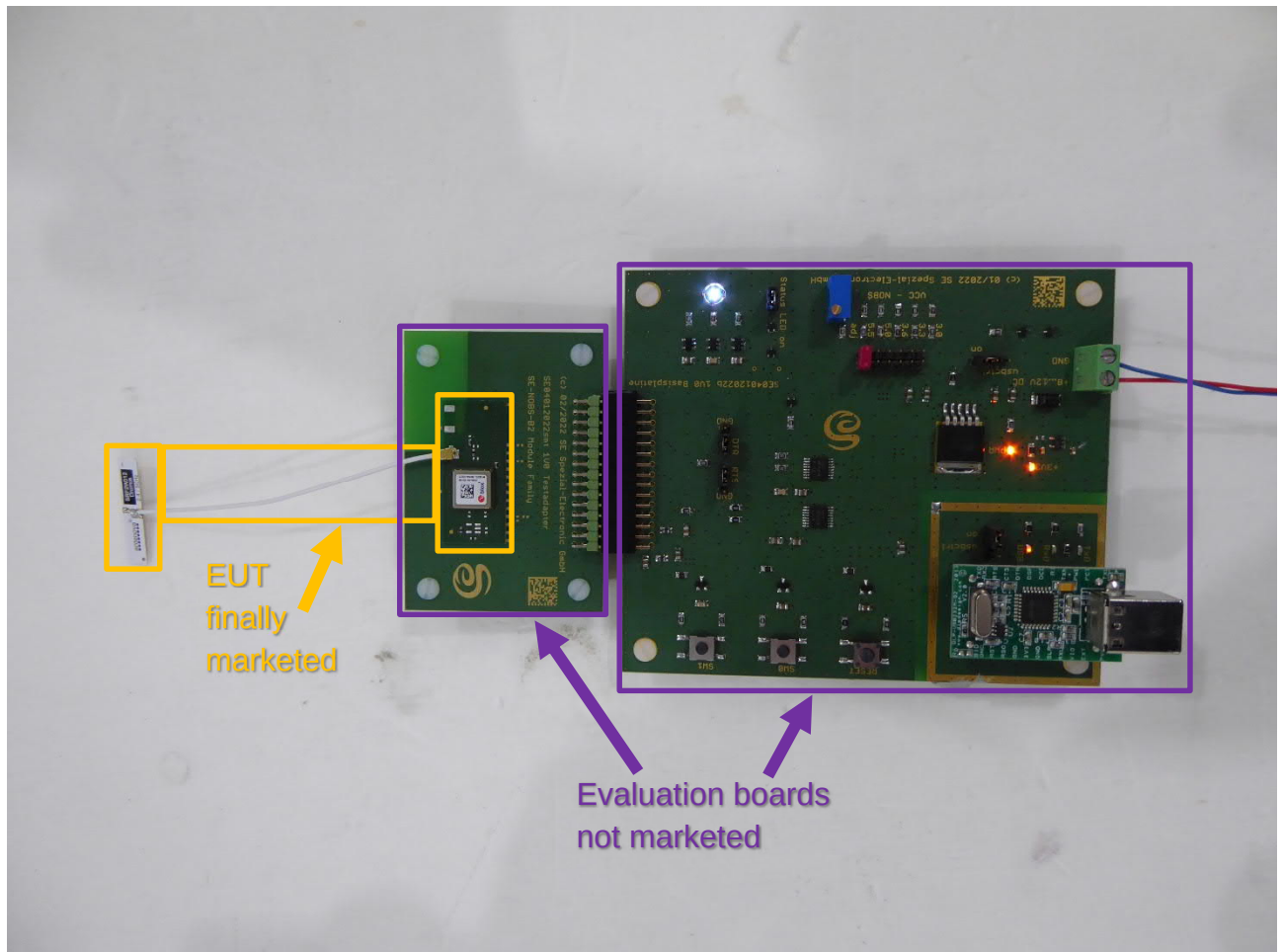
Test setup anechoic chamber (#44)
