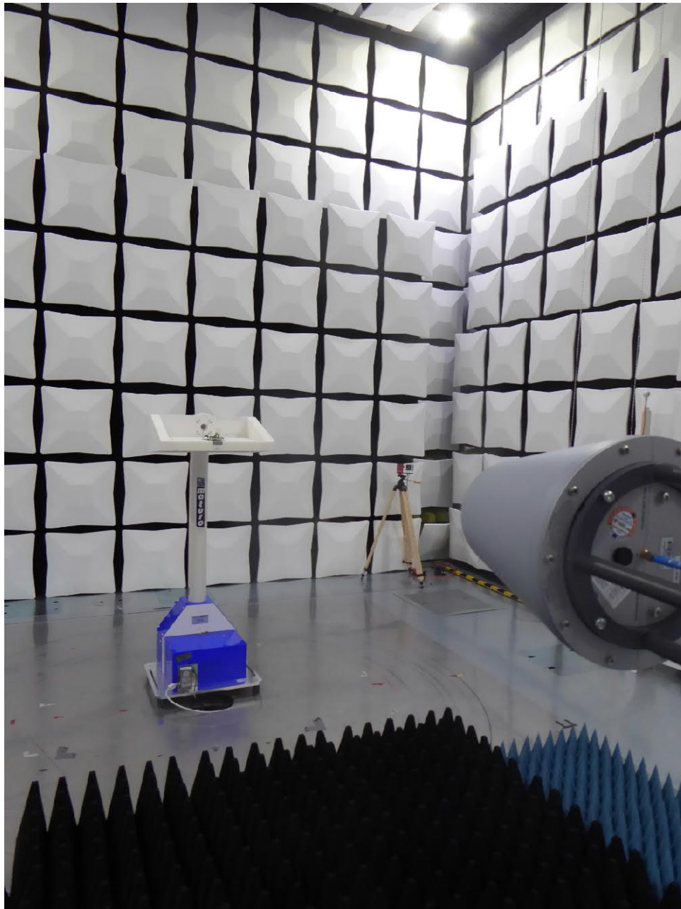
Test setup anechoic chamber (#44)
