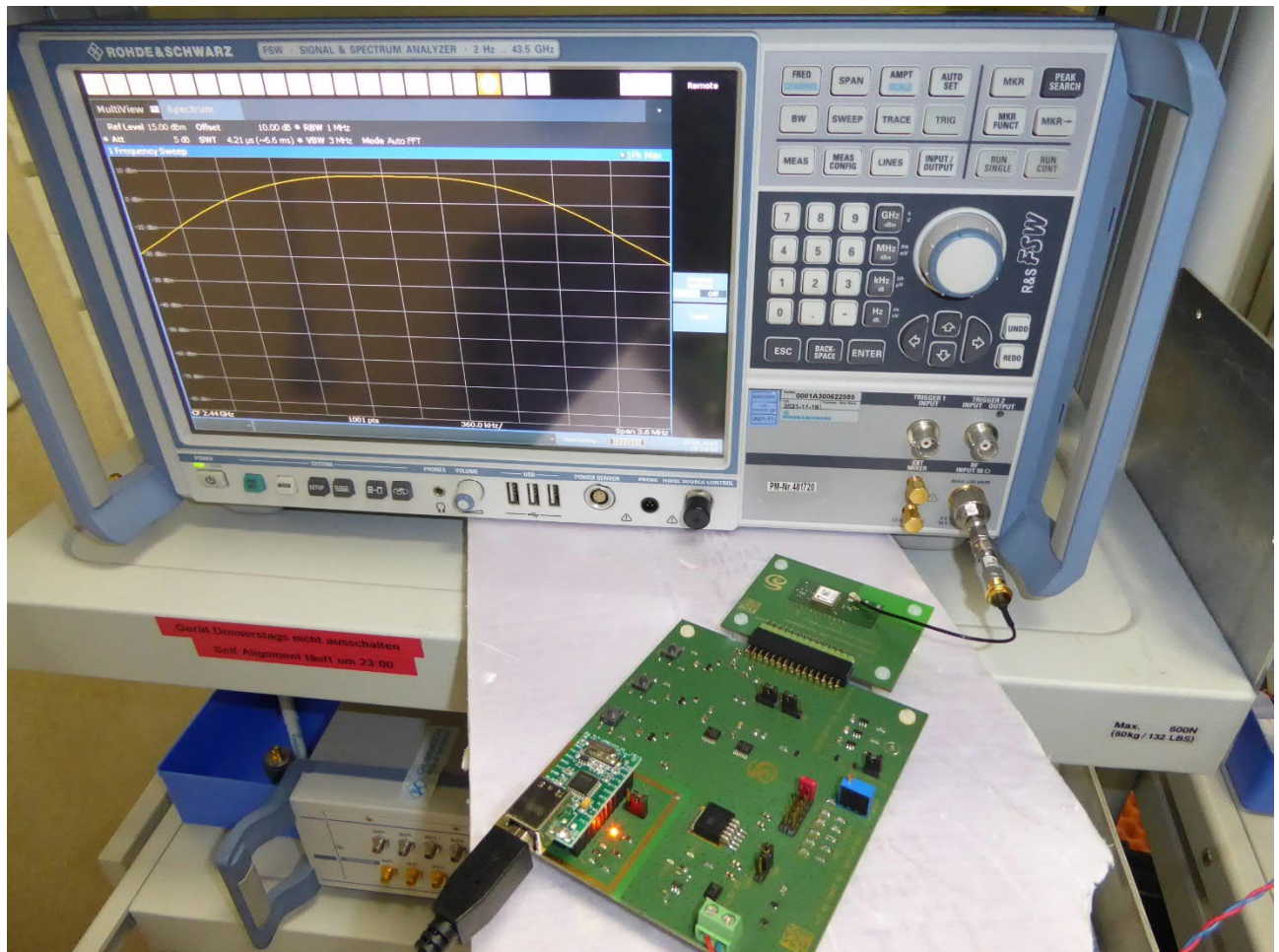
Test setup – antenna port conducted (EUT #44)
