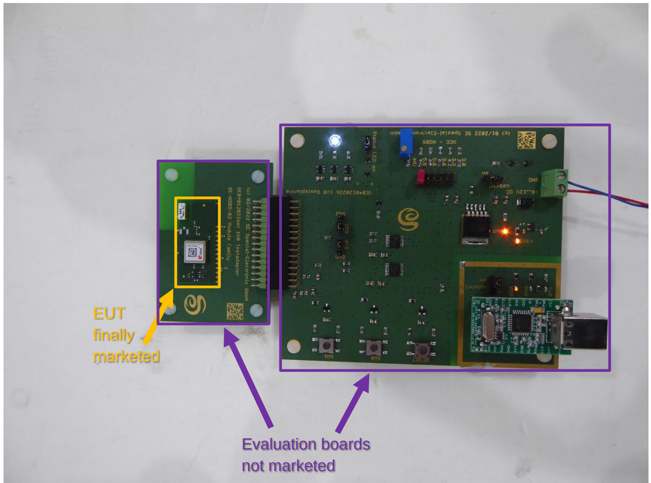
Test setup anechoic chamber (#41)
