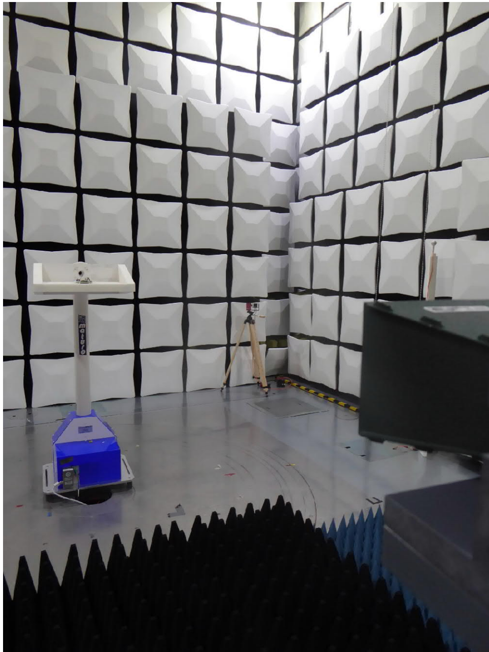
Test setup anechoic chamber (#41)
