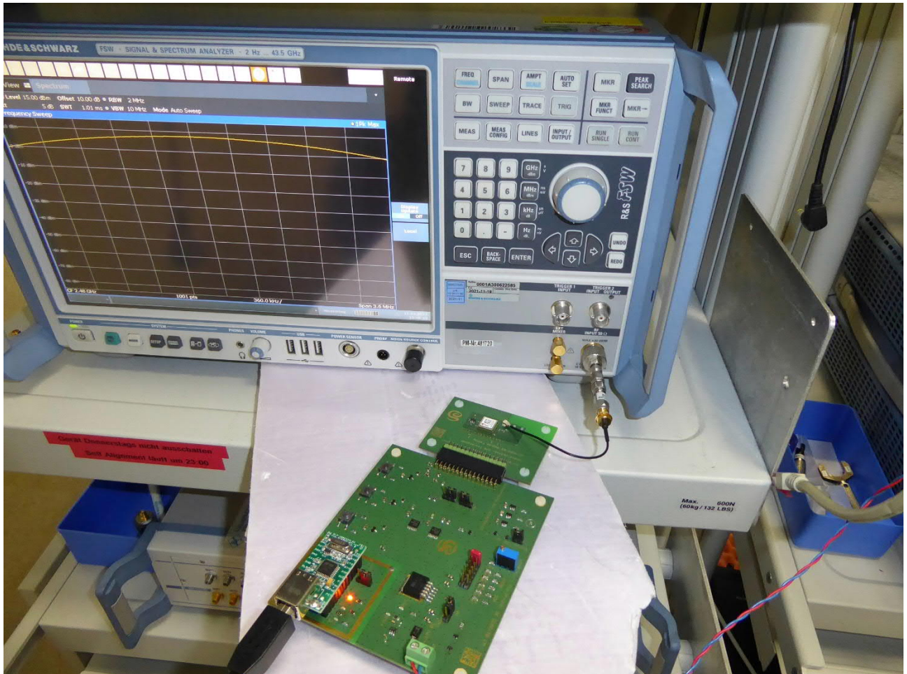
Test setup – antenna port conducted (EUT #48)
