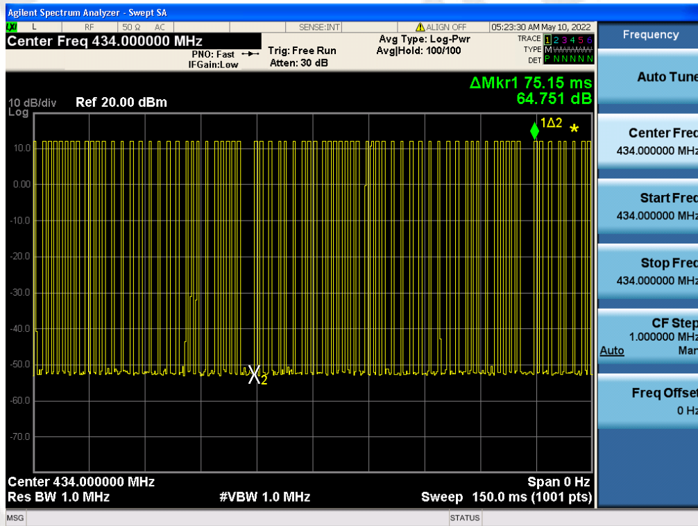
(Transmit cycle 75.15ms)
