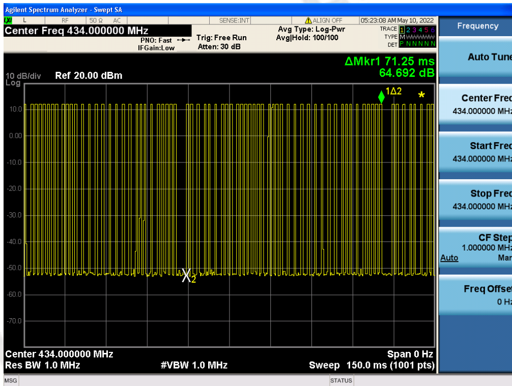
(Total Bursts in a transmit cycle 37pcs)
